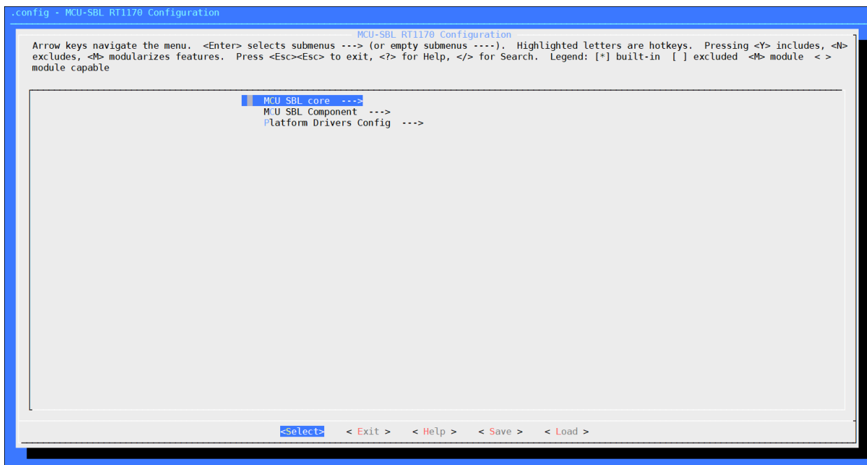
图12. SBL配置菜单
