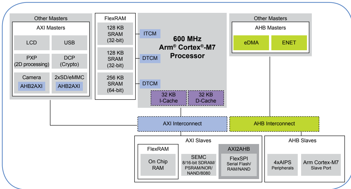
Figure 6: i.MX RT Architecture Diagram
