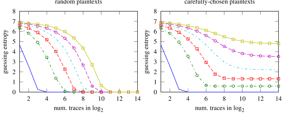
Figure 1.3: Average guessing entropy after attacks with known plaintexts for N_s = 1 (blue,s/), 2 (green,dd/c), 4 (red,d/s), 8 (cyan,dd/), 16 (magenta,d/c), and 32 (yellow,s/s) with \{s=\text{solid}, d=\text{dashed}, dd=\text{dotted dashed}\}/\{c=\text{circle}, s=\text{square}\} .
