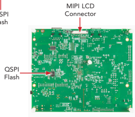
Figure 2: MIMXRT1170-EVKB Board Back Callouts
