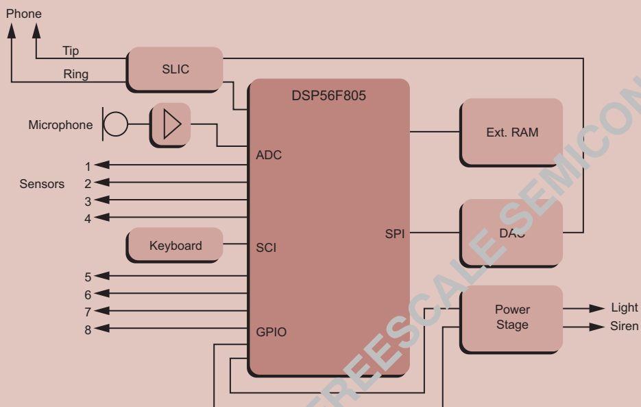
BLOCK DIAGRAM OF LIGHT AND HEATING CONTROL USING DSP56F805 WITH INTEGRATED SIMPLE VOICE CONTROL
