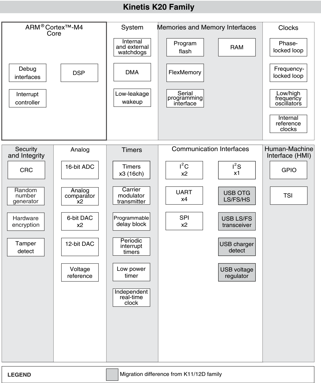
Figure 2. K20 Block Diagram
