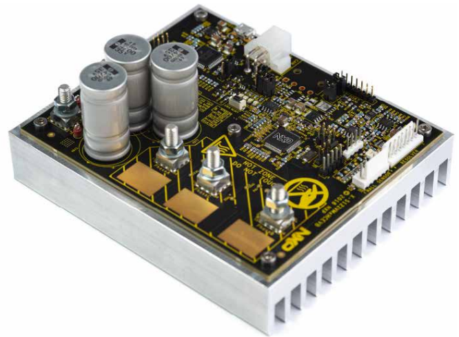
3-PHASE MOTOR CONTROL HIGH-CURRENT EVALUATION BOARD WITH S12ZVM
