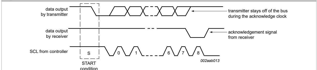
Figure 15. Acknowledge on the I 2 C-bus
