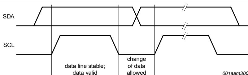
Figure 14. Bit transfer on the I 2 C-bus.
