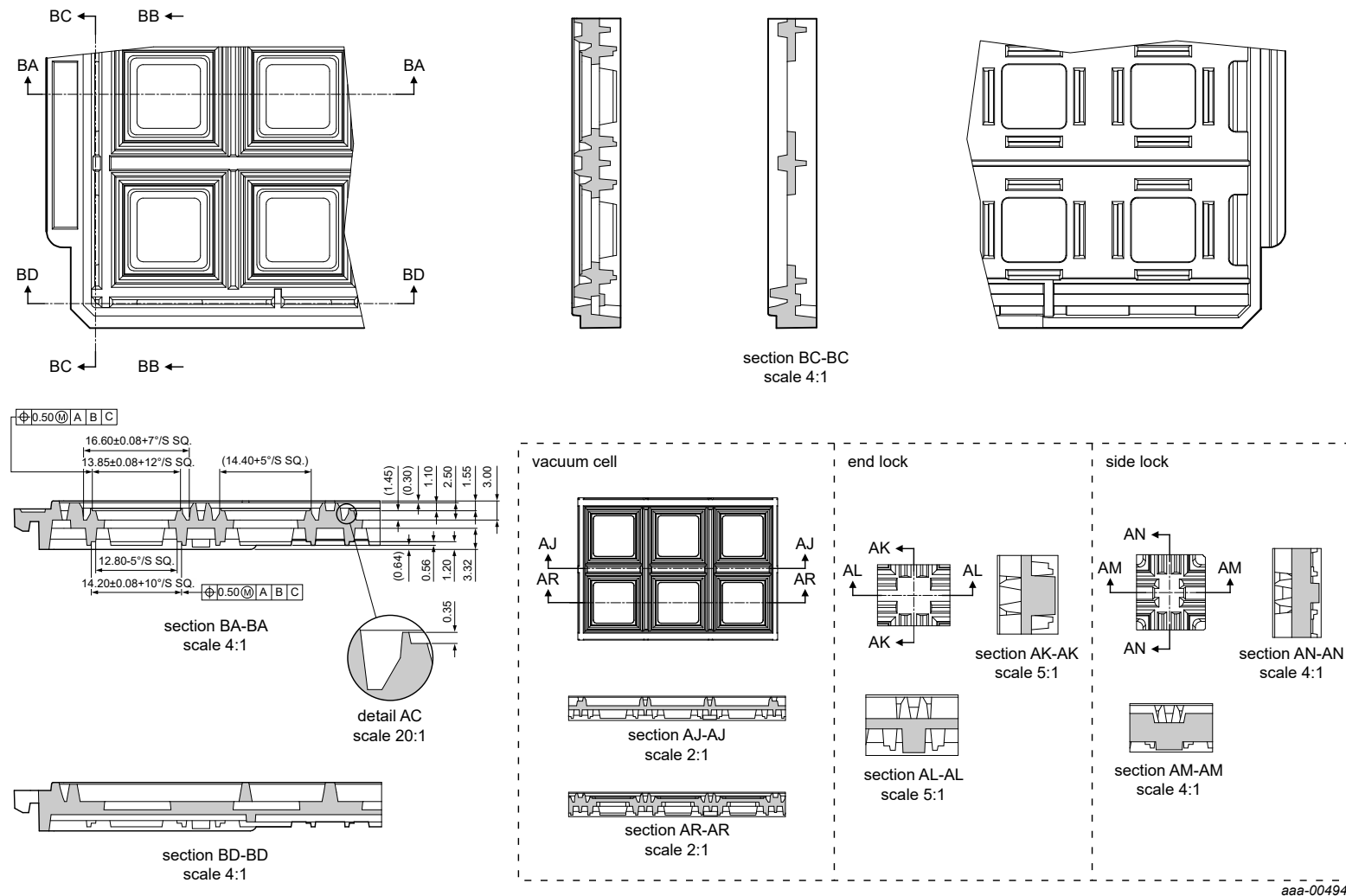
Figure 37. Tray details
