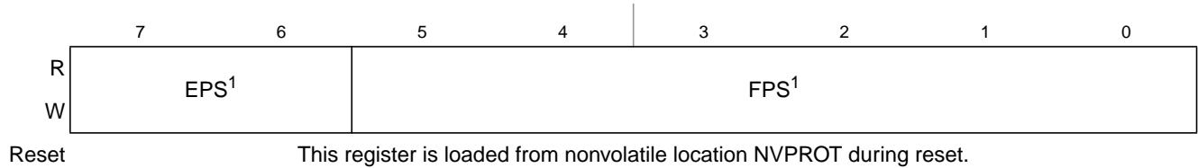
Figure 4-9. Flash and EEPROM Protection Register (FPROT)
