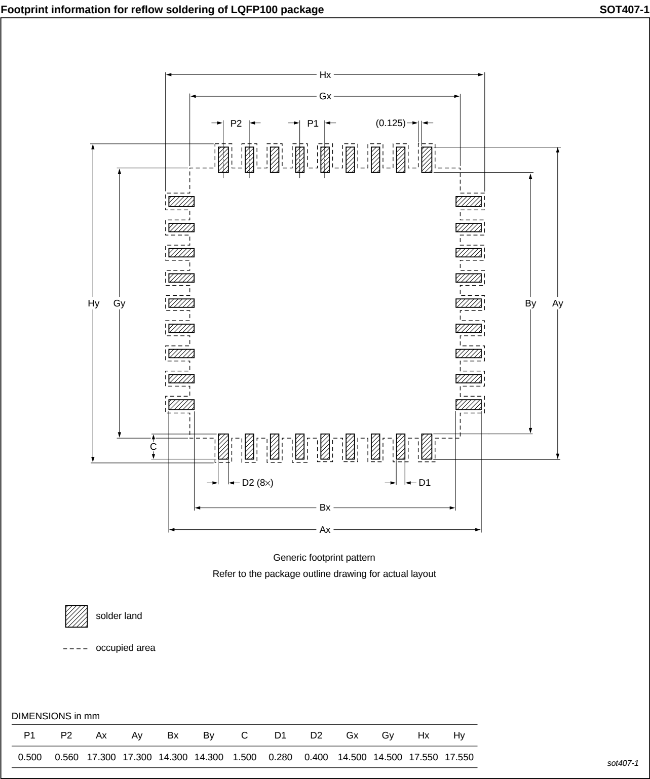
Fig 55. Reflow soldering of the LQFP100 package
