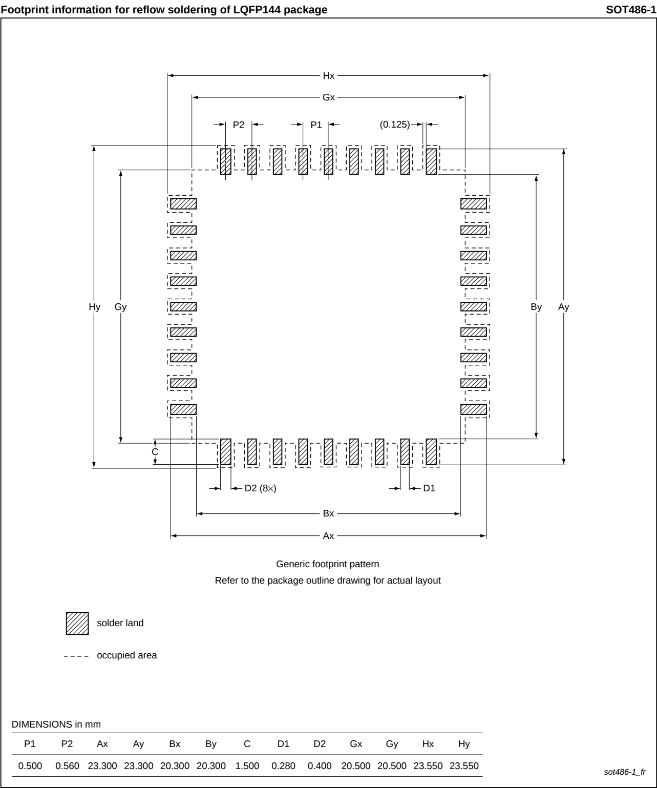
Fig 54. Reflow soldering of the LQFP144 package
