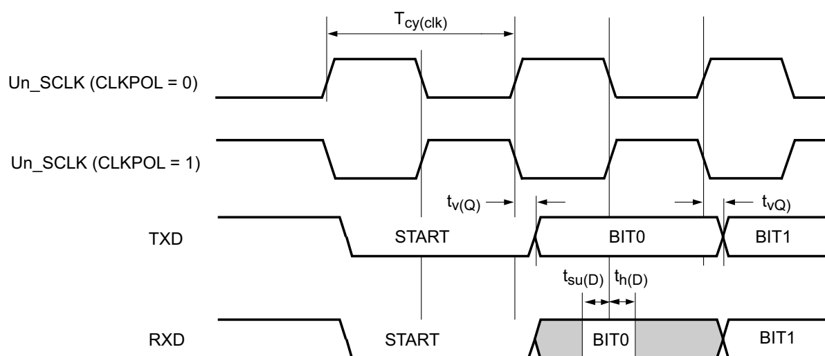
Fig 17. USART interface timings
