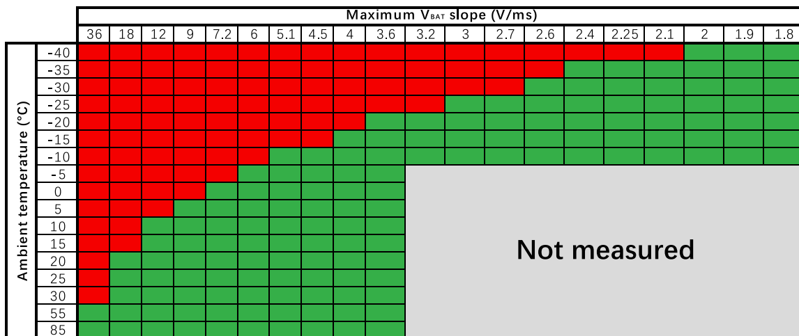
Fig 12. Maximum V_{BAT} slope vs temperature
