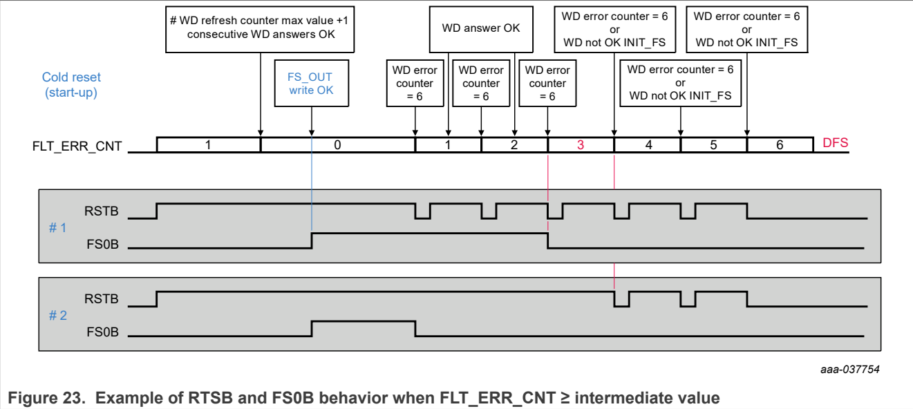
Figure 23. Example of RSTB and FS0B behavior when FLT_ERR_CNT ≥ intermediate value
