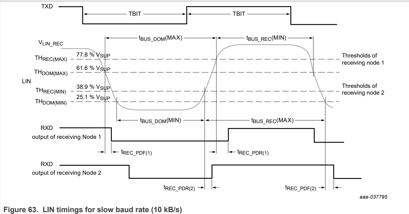
Figure 63. LIN timings for slow baud rate (10 kB/s)
