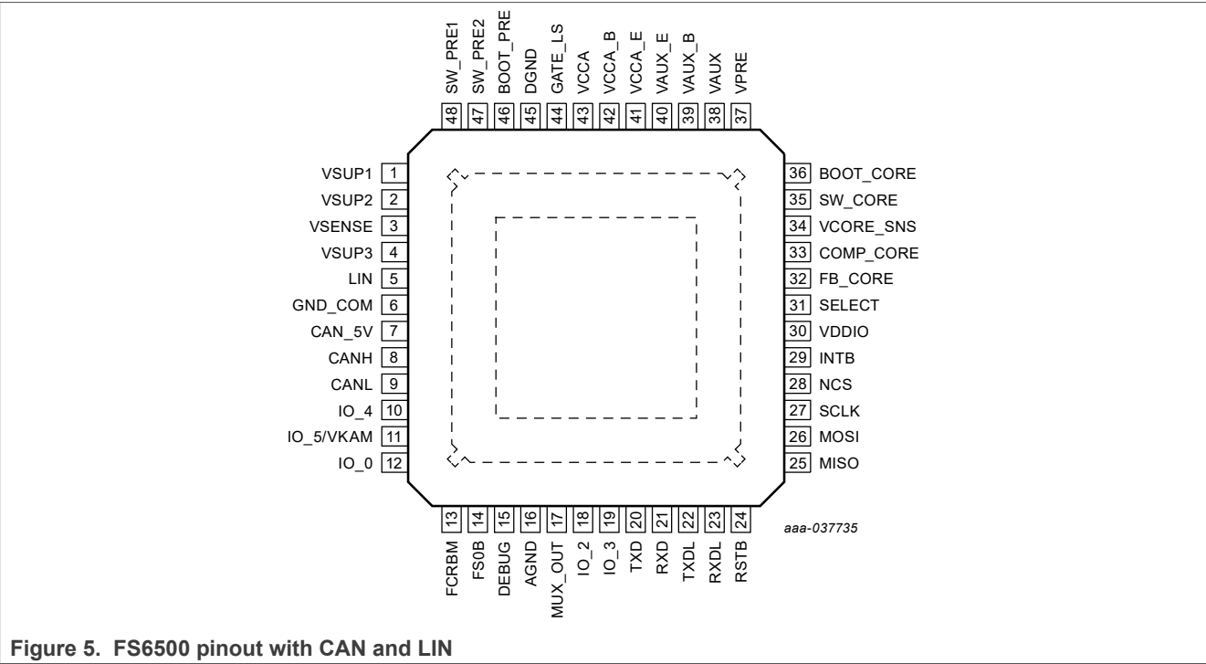
Figure 4. FS6500 pinout with CAN and FS1B
