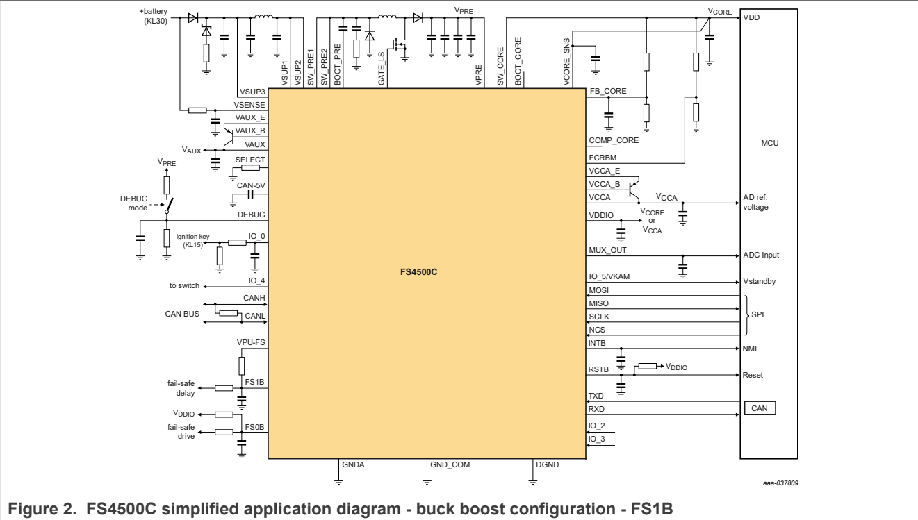
Figure 2. FS4500C simplified application diagram - buck boost configuration - FS1B
