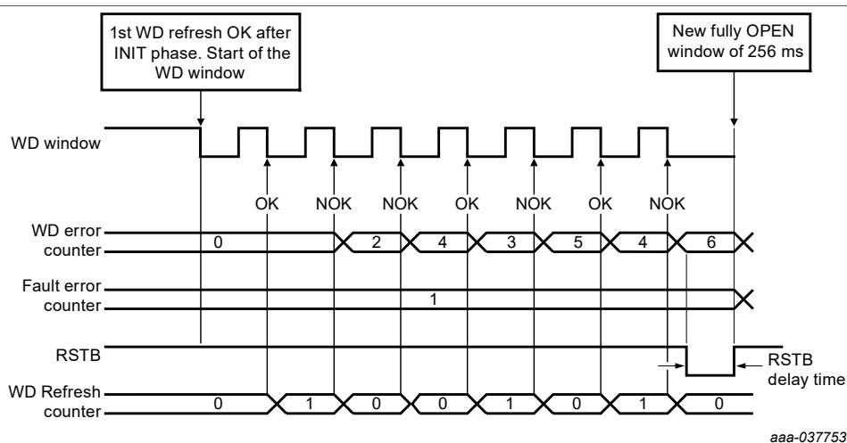
Figure 22. Example of WD operation generating a reset (WD_CNT_ERR = 6)
