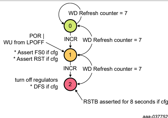
Figure 21. Fault error counter (FLT_ERR_FS = 1, WD_CNT_RFR = 6)
