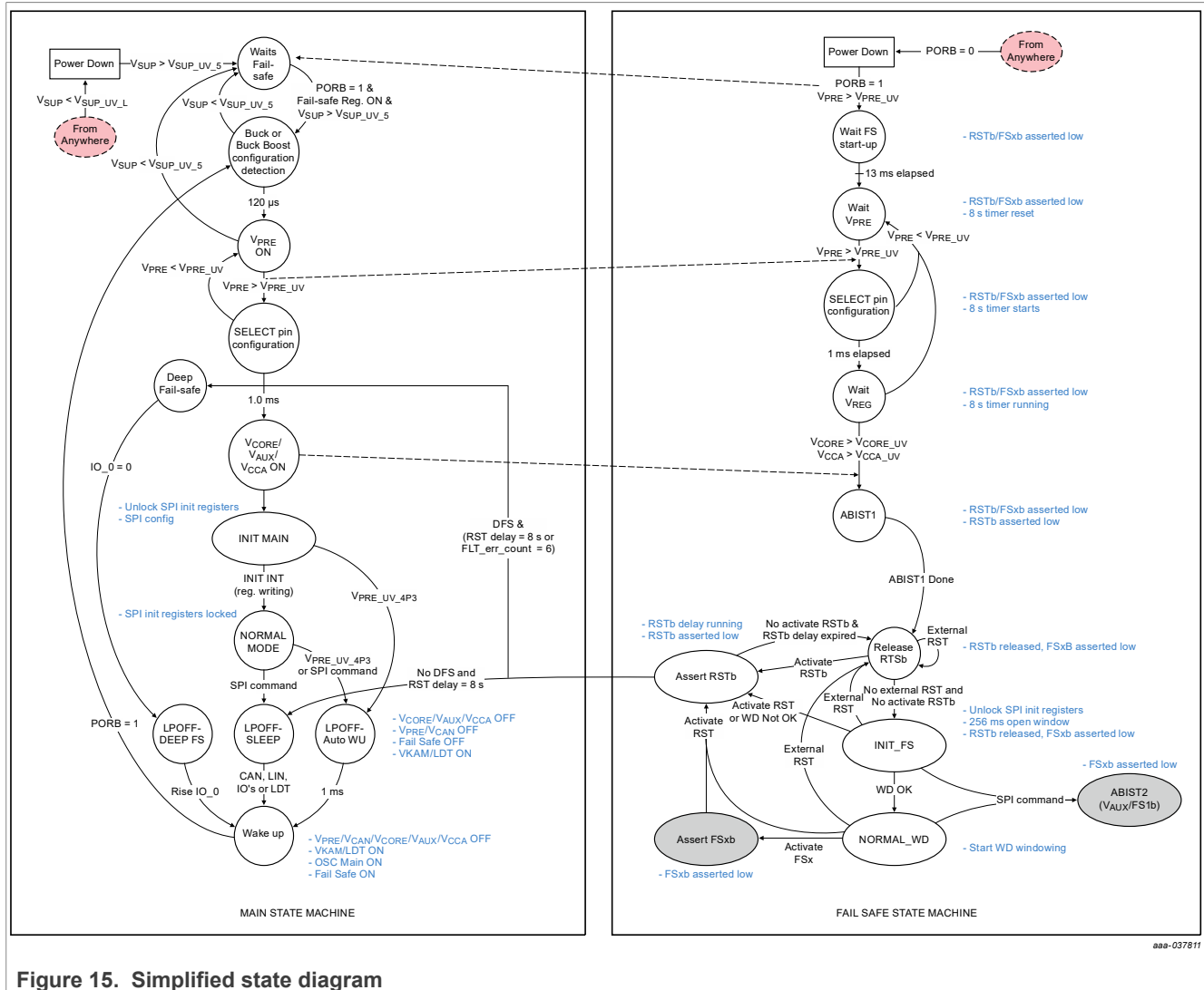
Figure 15. Simplified state diagram
