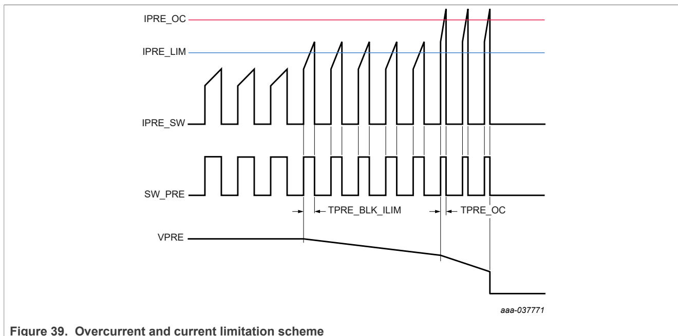
Figure 39. Overcurrent and current limitation scheme
