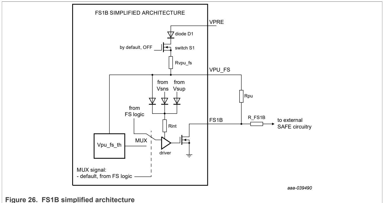
Figure 26. FS1B simplified architecture
