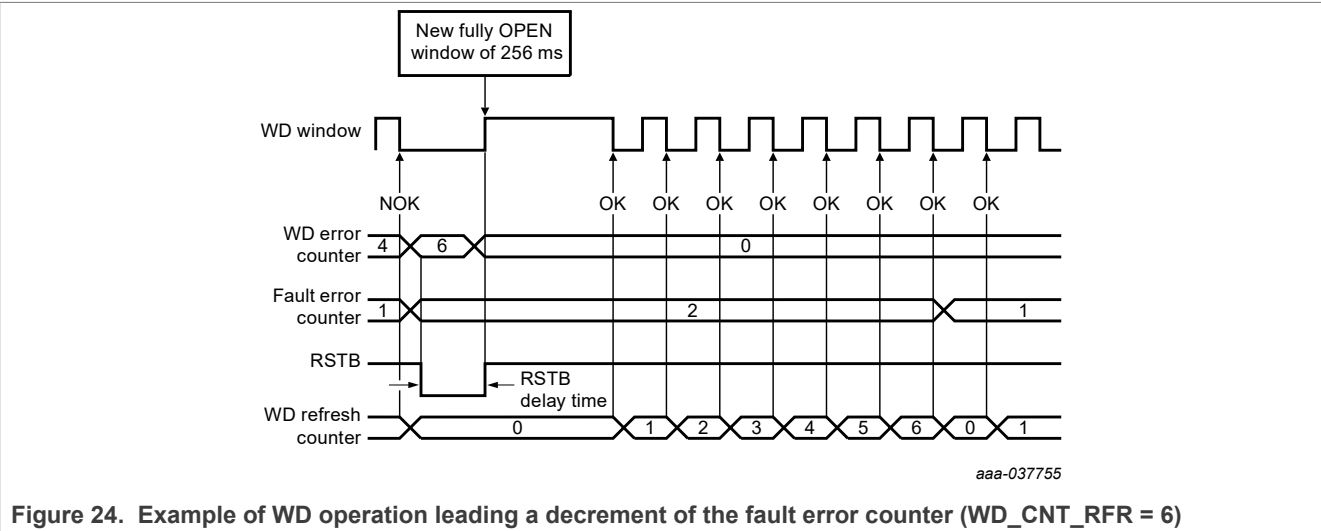
Figure 24. Example of WD operation leading a decrement of the fault error counter (WD_CNT_RFR = 6)
