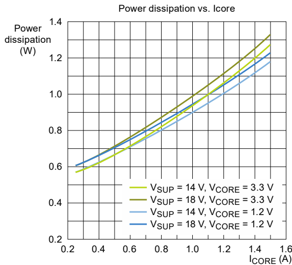
Figure 49. Power dissipation versus I_{CORE} , I_{CCA} , or I_{PRE}
