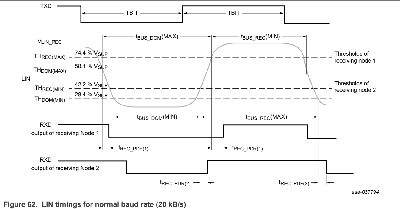
Figure 62. LIN timings for normal baud rate (20 kB/s)
