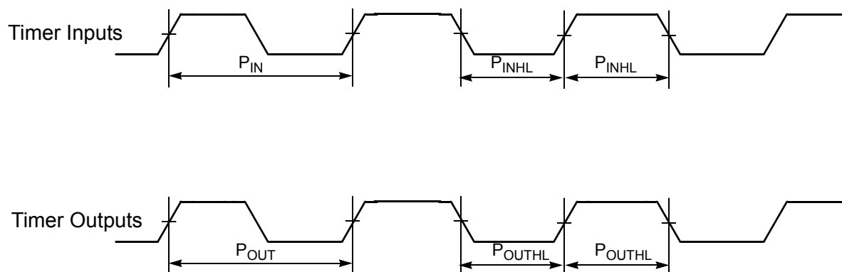
Figure 4-21 Timer Timing
