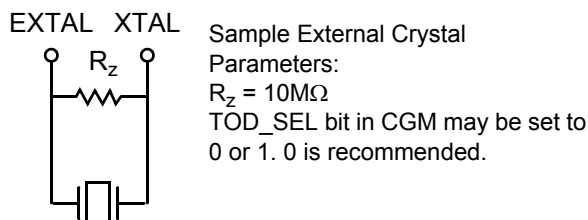
Figure 4-6 Crystal Oscillator
