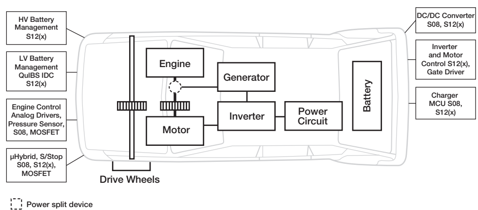
PHEV Reference Diagram
