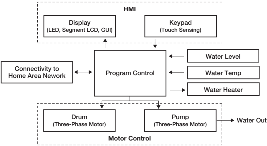
Washing Machine Block Diagram
