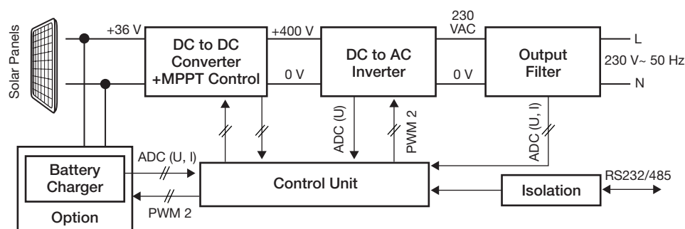
Photovoltaic System Block Diagram
