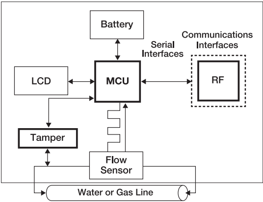
Flow Meter Block Diagram
