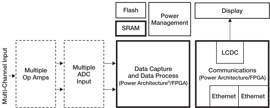
Power Breaker Controller Block Diagram
