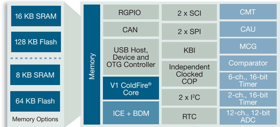
MCF51JM128 Block Diagram
