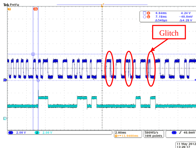
Figure 21. Bit receiving wave with anti-jamming algorithm
