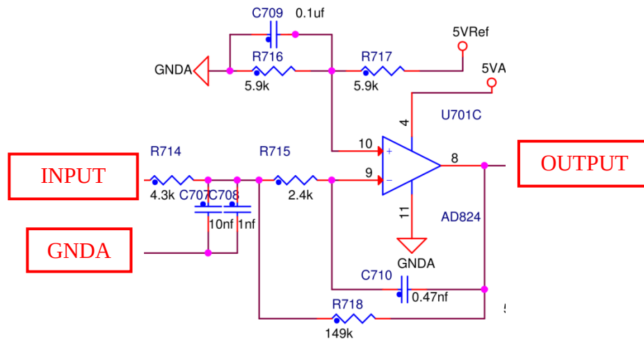
Figure 11. Low-pass filter
