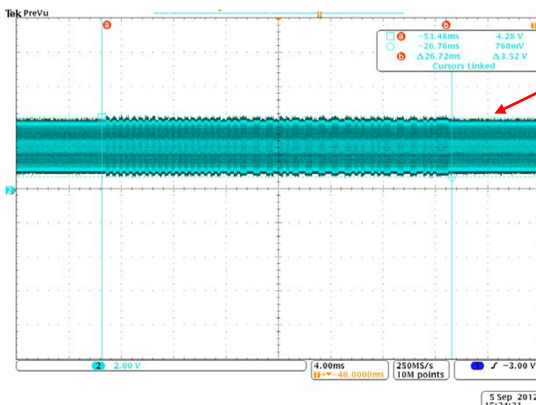
Figure 8. Communication wave after the voltage scale down circuit
