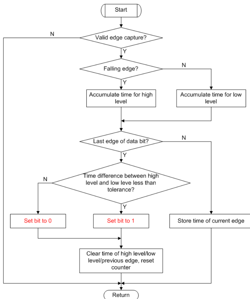
Figure 20. Optimized anti-jamming algorithm flowchart
