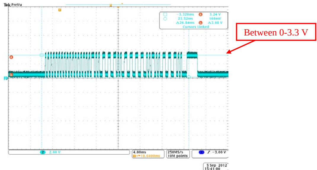
Figure 17. Communication wave after the voltage divider circuit
