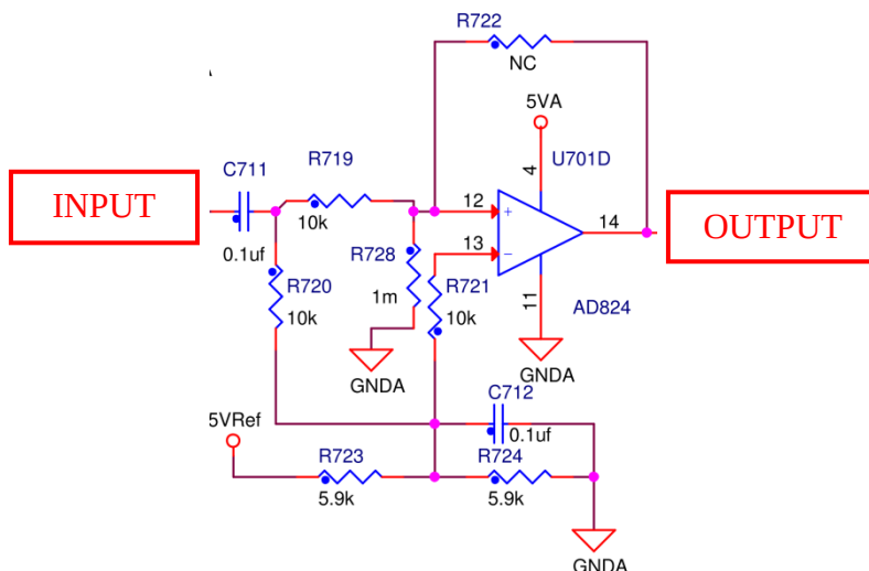
Figure 14. Comparator circuits
