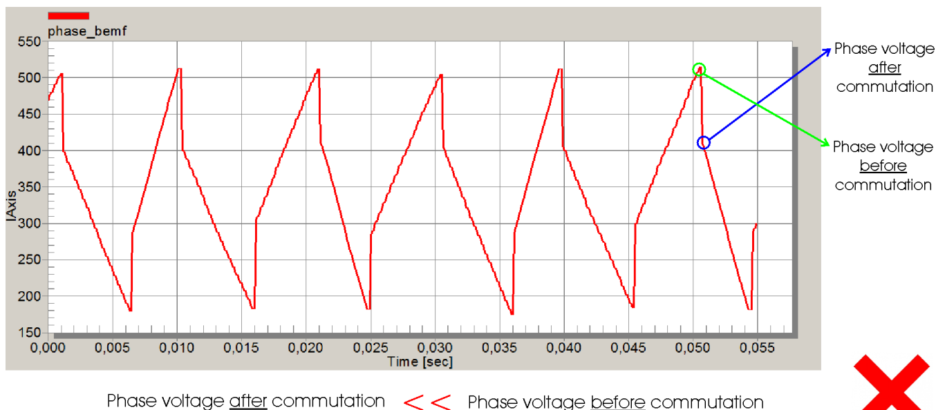
Figure 8. Late commutation timing
