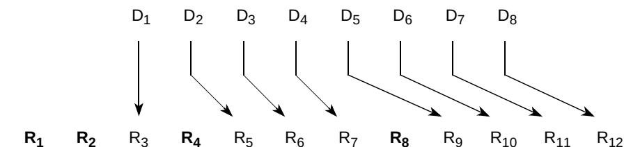
Figure 1. Encoding an 8-bit Data Vector into an SECDED ECC Codeword
