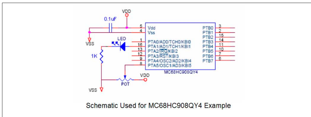
Figure 5. Schematic Used for MC68HC908QY4 Example
