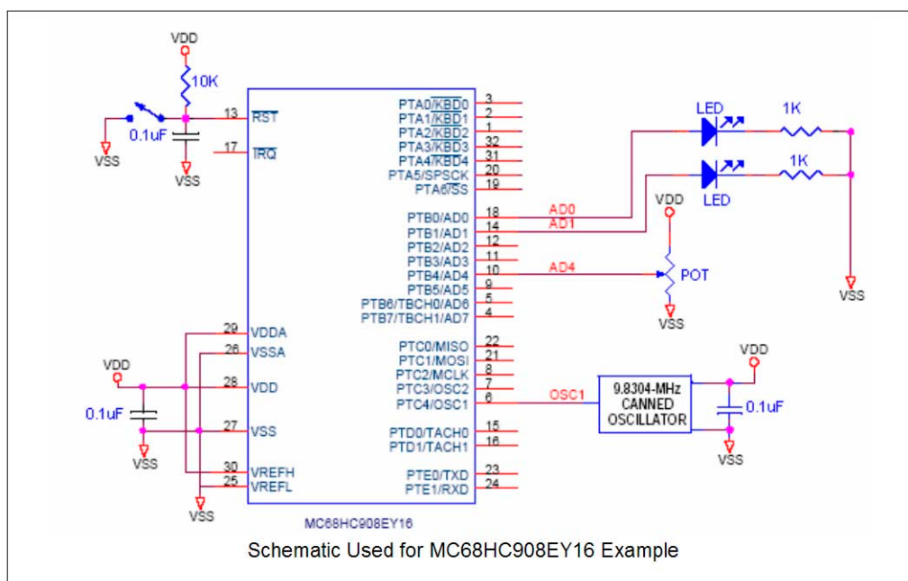
Figure 4. Schematic Used for MC68HC908EY16 Example
