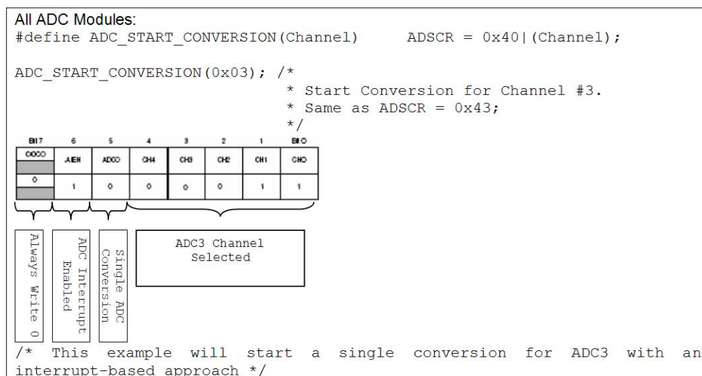
Figure 2. Starting a Single ADC Conversion
