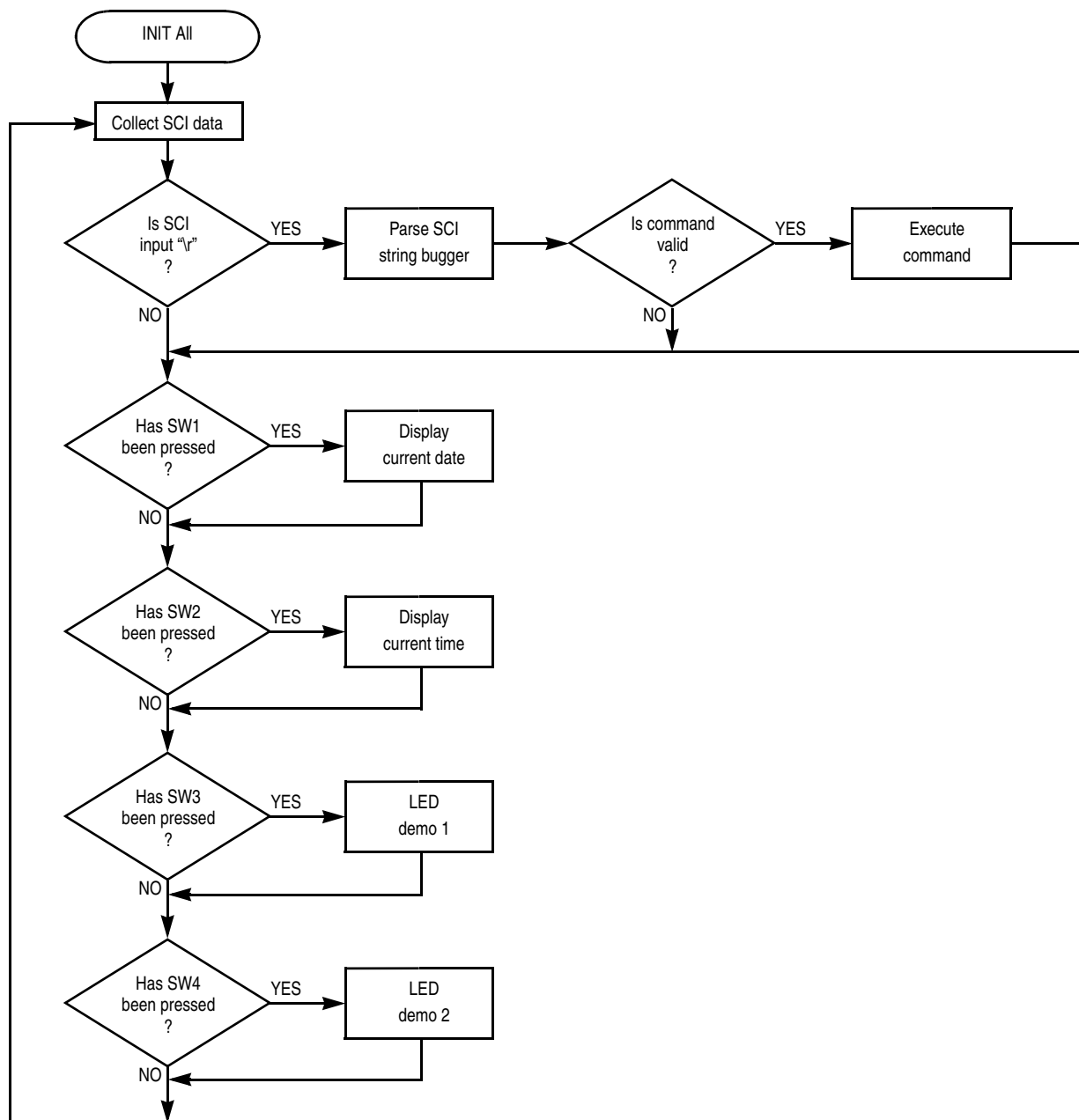
Figure 15. Main Flowchart
