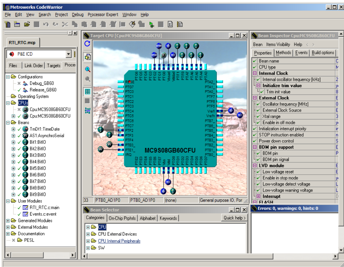
Figure 1. CodeWarrior IDE with Processor Expert Workspace
