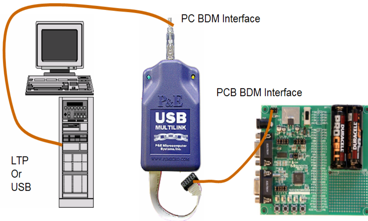
Figure 4. Development Environment Debugger/Programmer Connections
