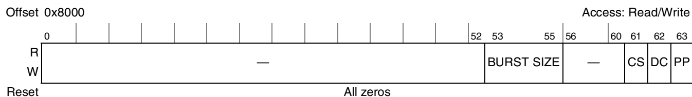
Figure 7. AFEU Mode Register
