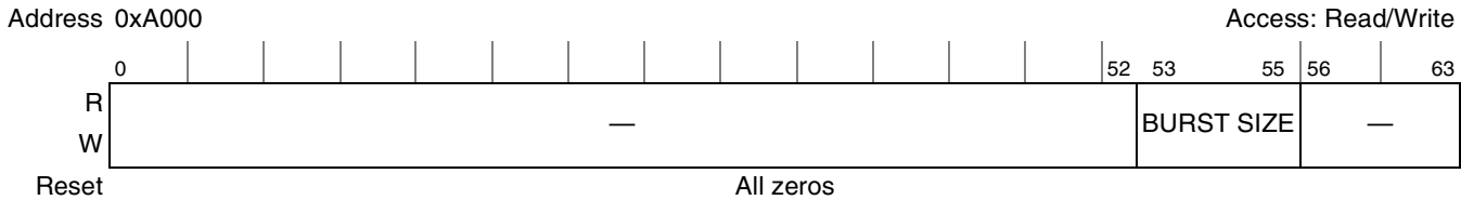
Figure 9. RNG Mode Register
