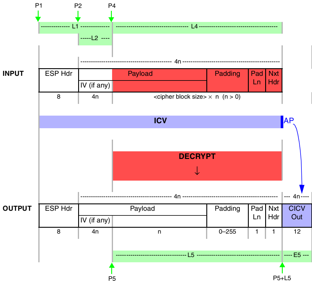
Figure 16. IPsec ESP Inbound Packet Pointer Diagram
