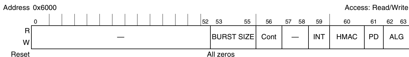
Figure 8. MDEU Mode Register
