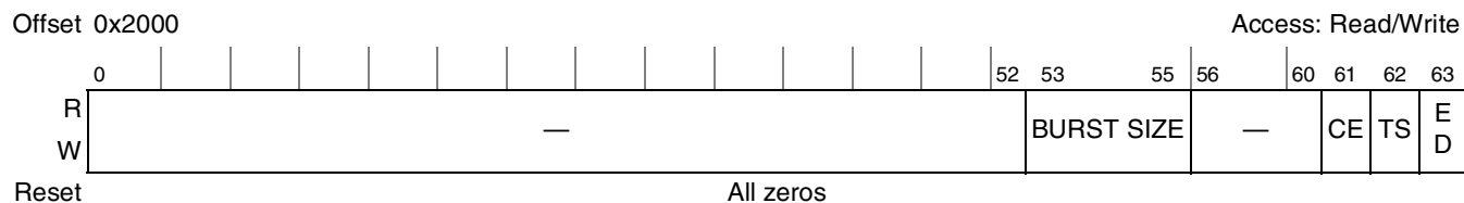
Figure 6. DEU Mode Register
