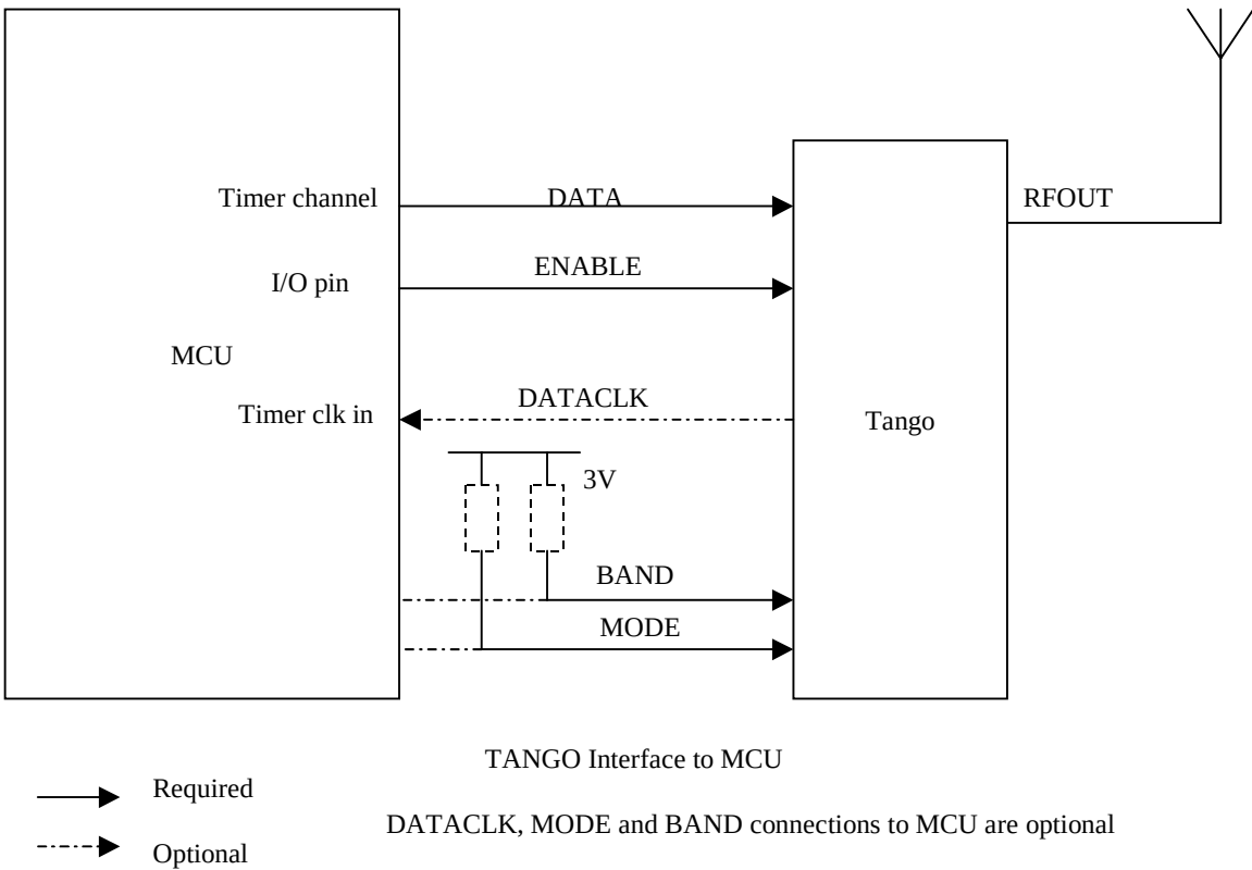
Figure 8. Tango3 Interface to MCU
