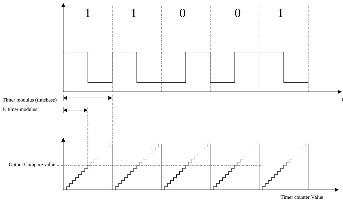
Figure 7. Bit Encoding Using MCU Timer Channel.
