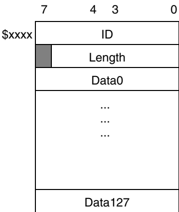
Figure 9. Tango3 Transmission Buffer
