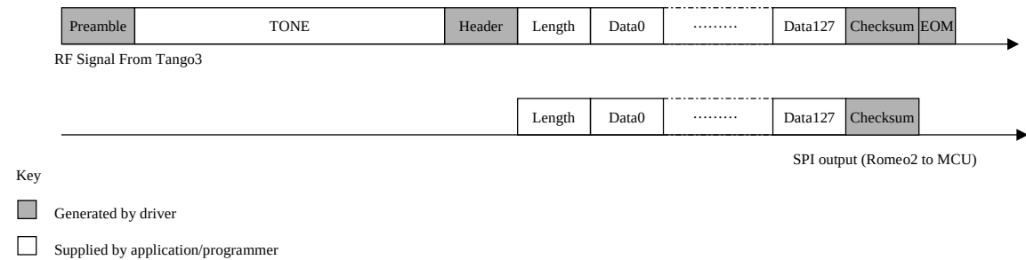
Figure 5. Message Format Using Tone Signalling
