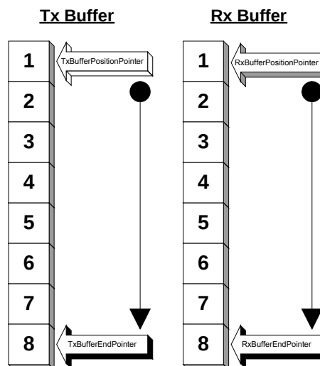
Figure 4. Transmit and Receive Buffer Arrangement
