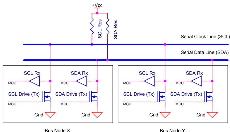
Figure 1. I²C Bus and Interface Hardware
