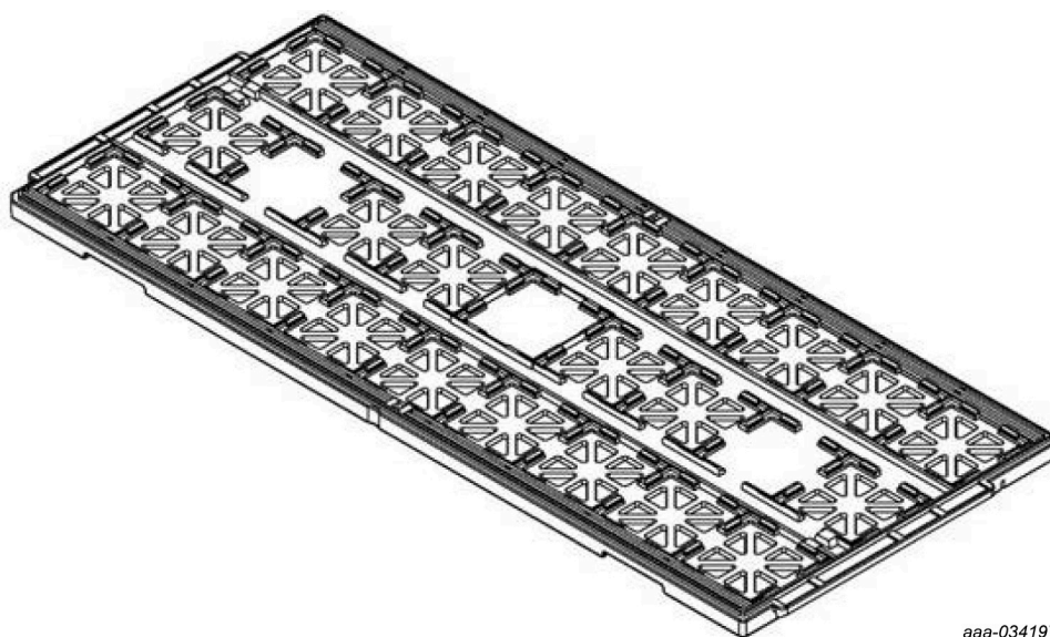
Figure 14. JEDEC tray example
