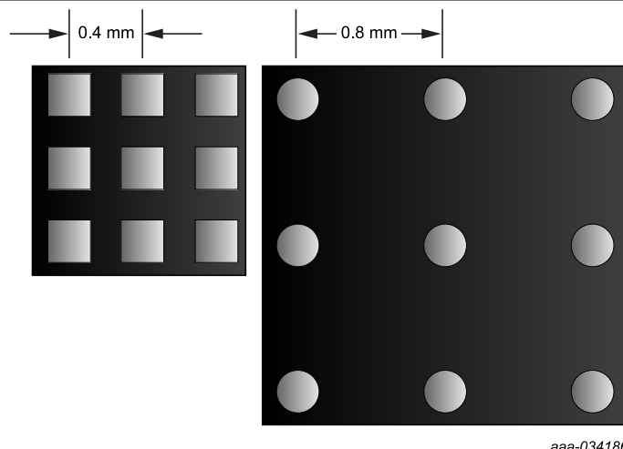
Figure 8. Square 0.4 mm and round 0.8 mm pitch stencil openings
