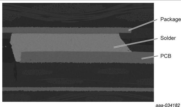
Figure 4. Scanning electron microscope (SEM) image of a well-soldered MAPLGA solder joint
