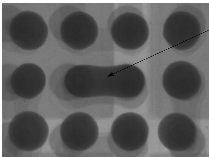
Figure 12. Two common LGA solder joint defects
