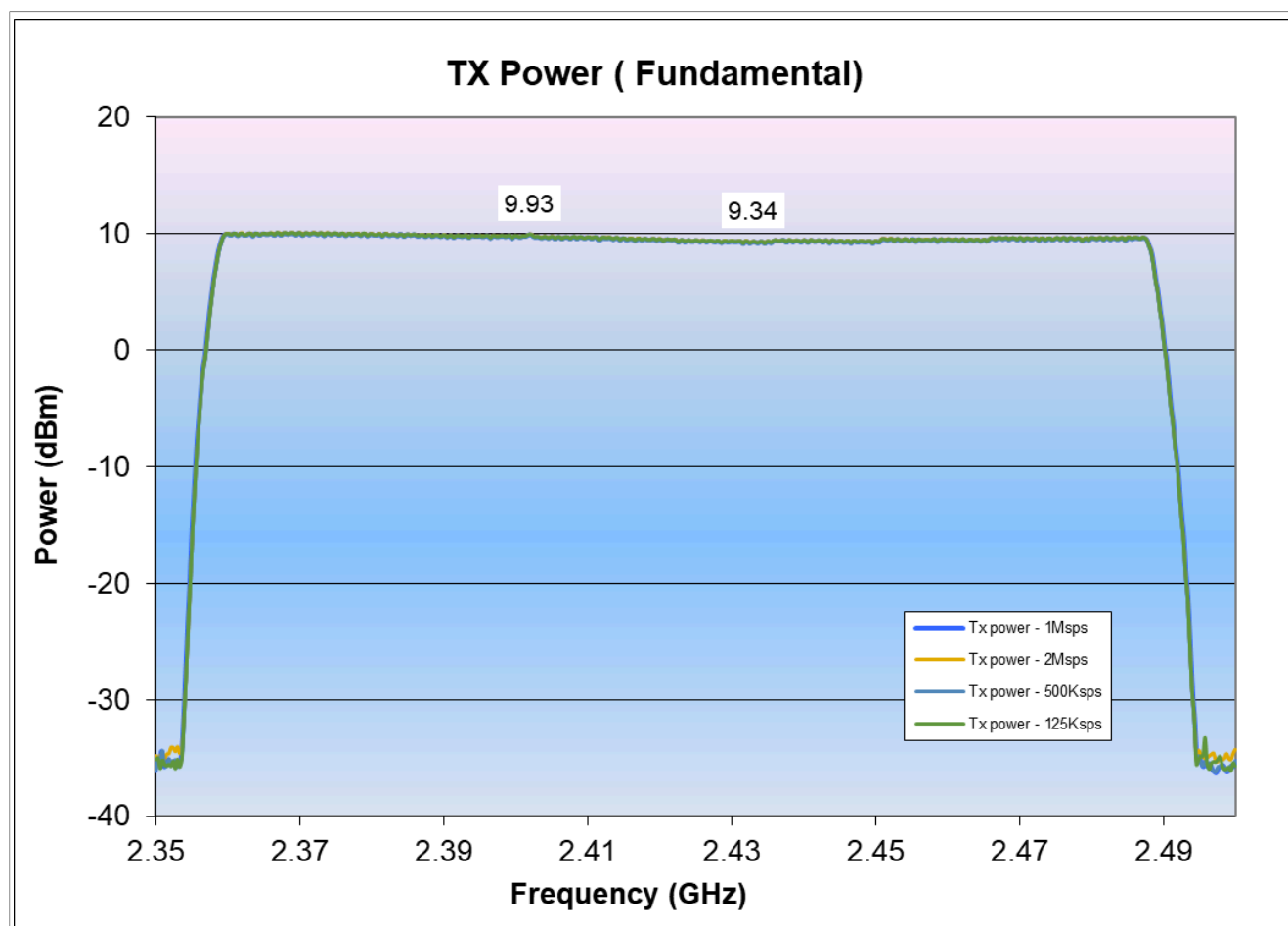
Figure 7. TX power
