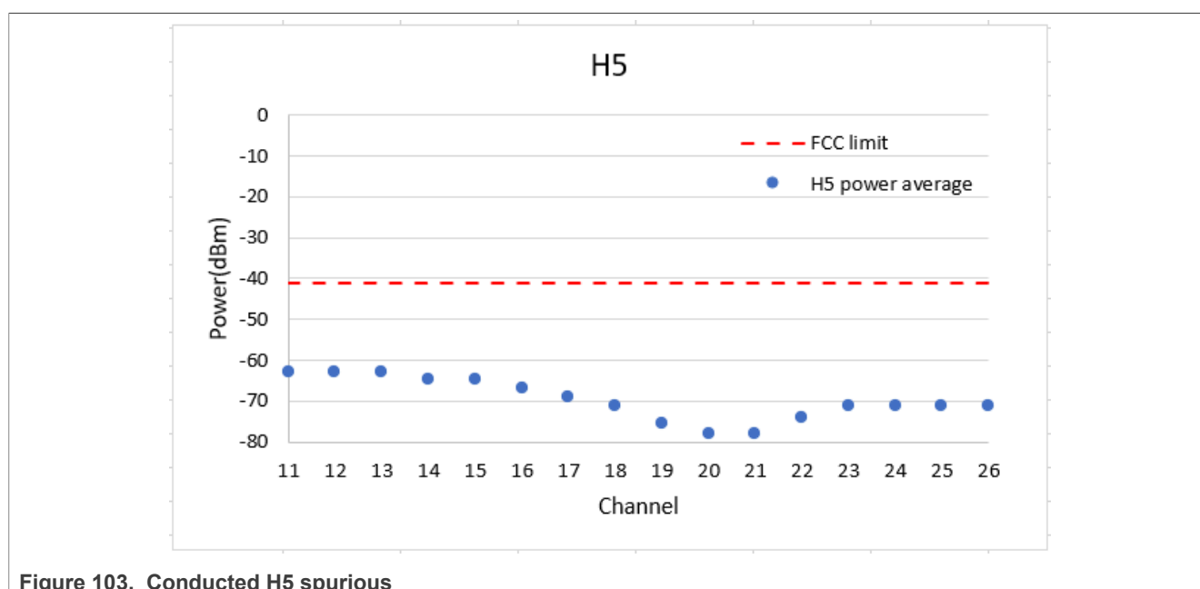
Figure 103. Conducted H5 spurious
