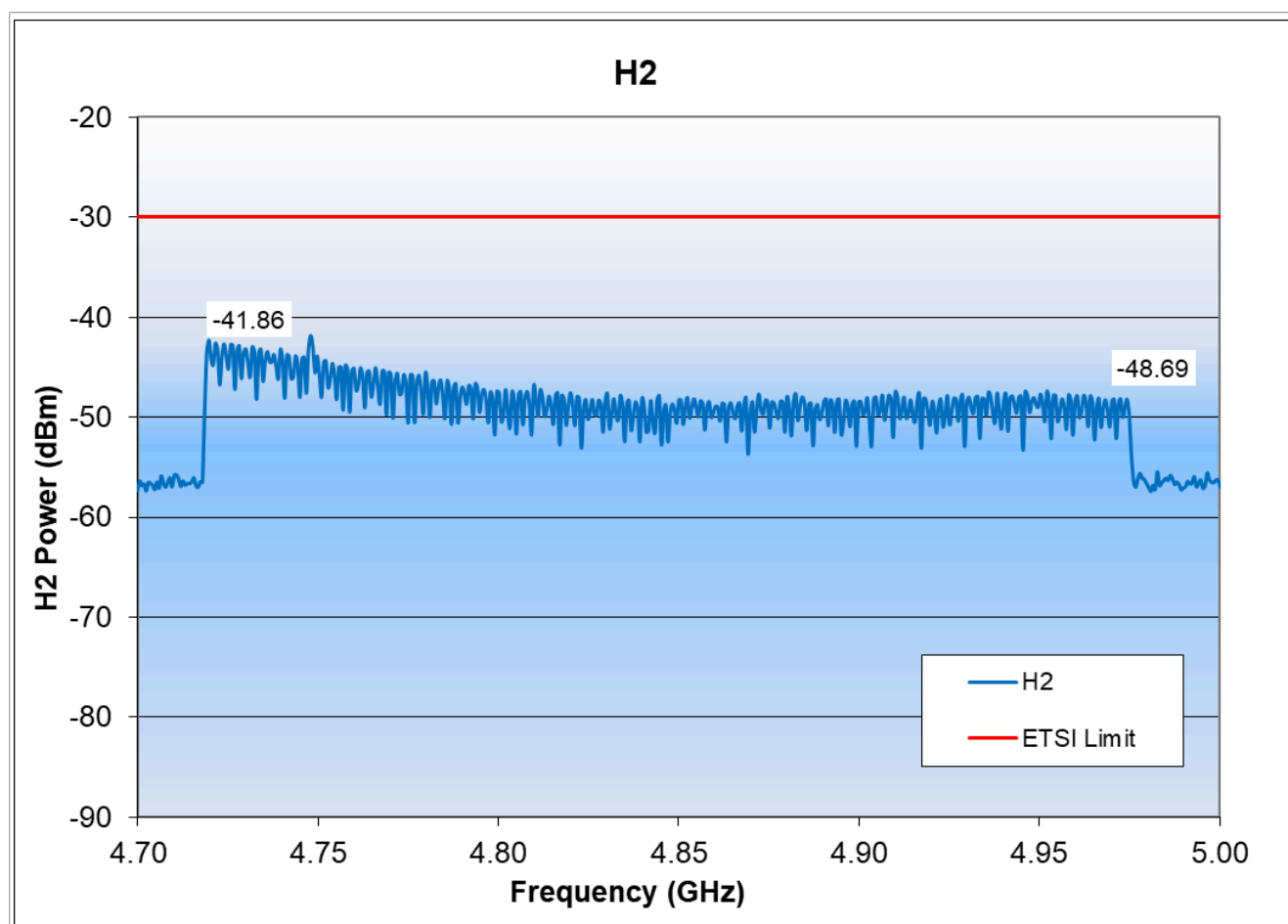
Figure 13. Bluetooth LE - Conducted H2 spurious
