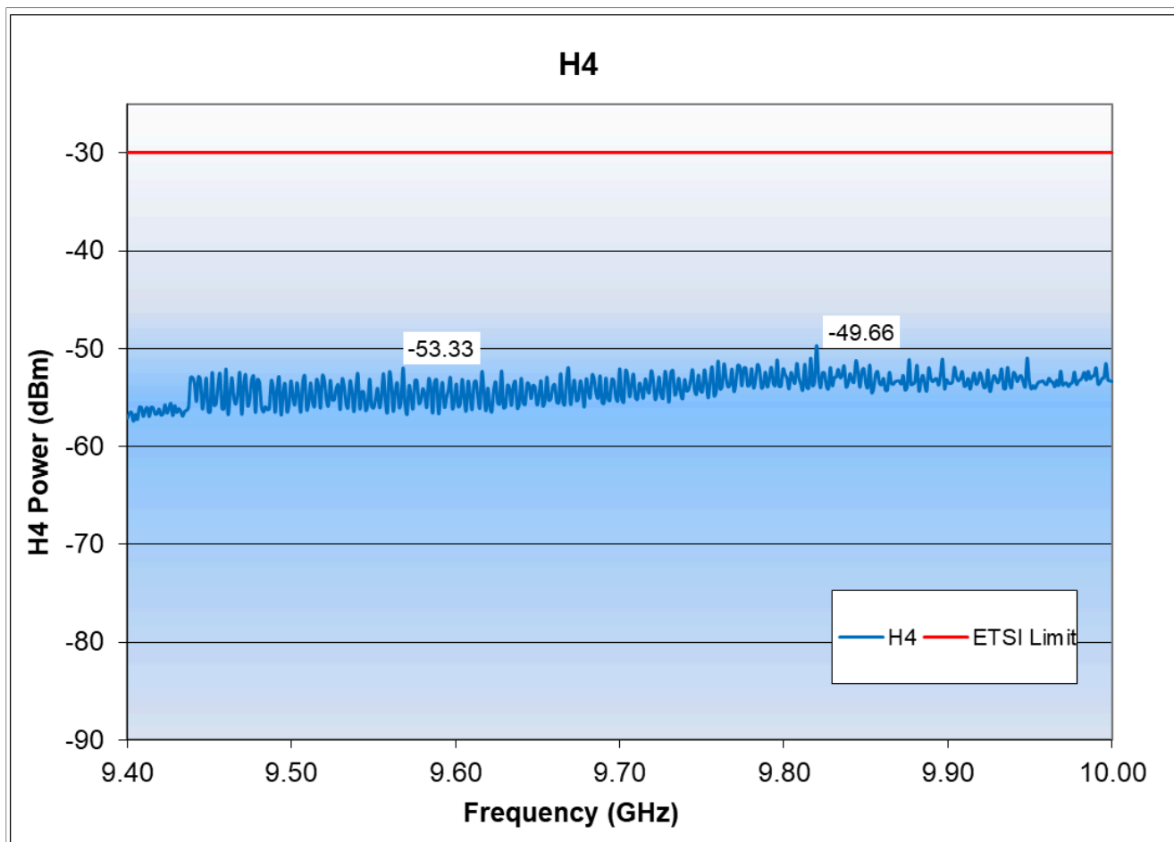
Figure 15. Bluetooth LE - Conducted H4 spurious
