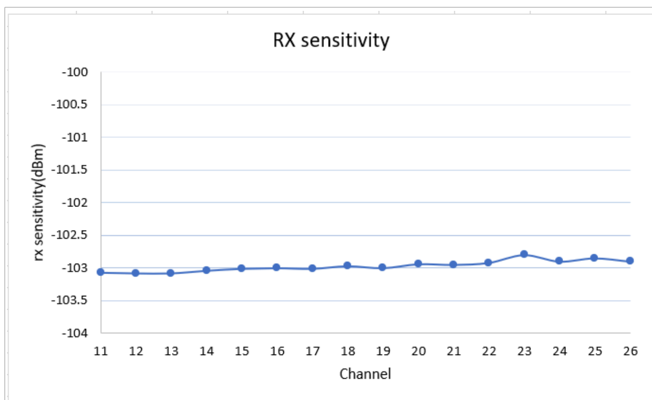
Figure 121. RX sensitivity
