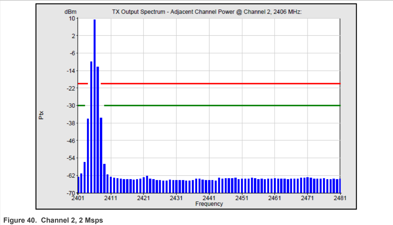
Figure 40. Channel 2, 2 Msps
