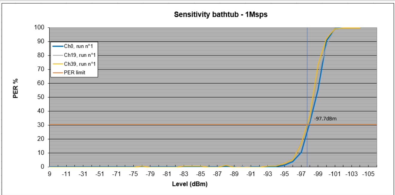
Figure 49. Sensitivity bathtub result – 1 Msps
