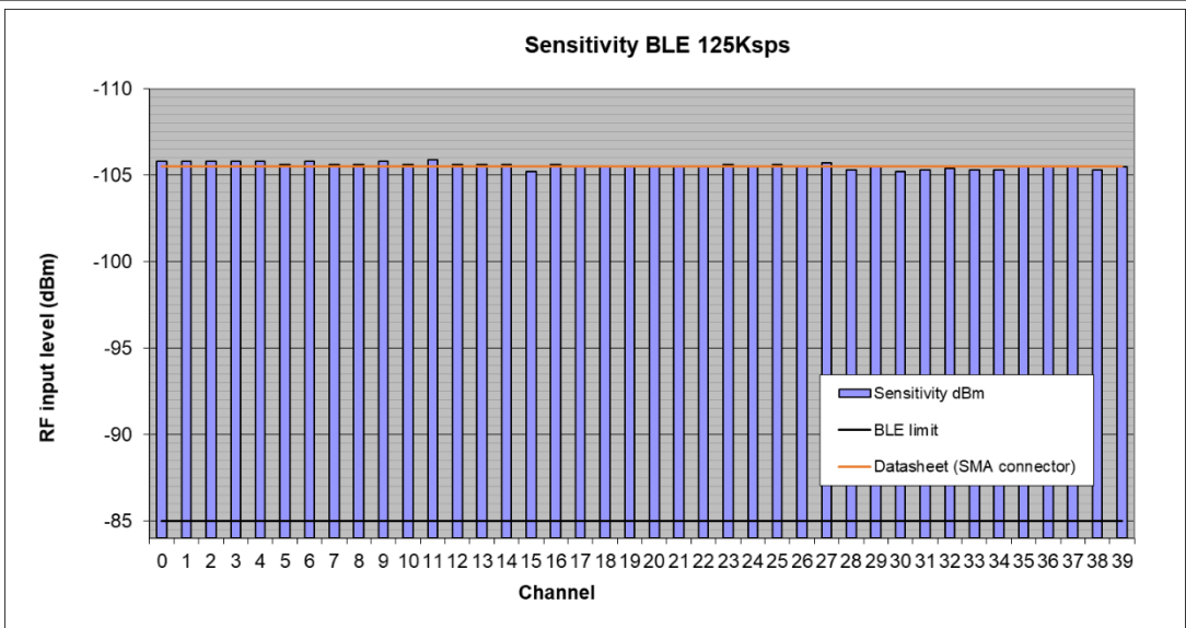
Figure 54. Sensitivity result – LR (S = 8)
