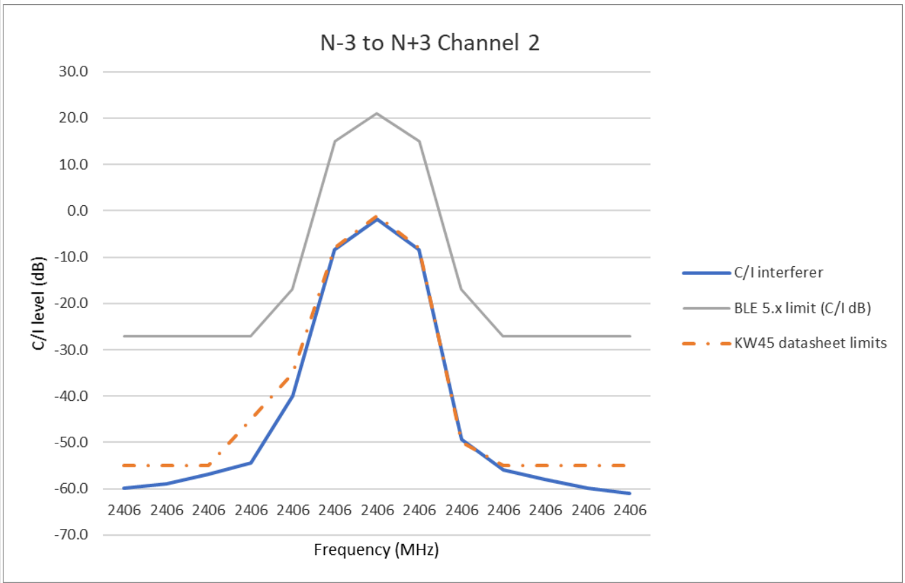
Figure 70. Adjacent, alternate, and co-channel rejection Bluetooth LE @125 ksps (LR S = 8) channel 2
