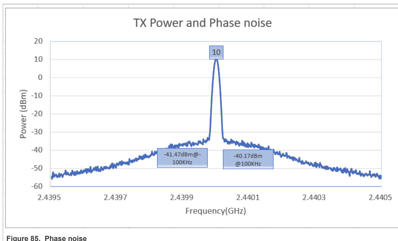
Figure 85. Phase noise
