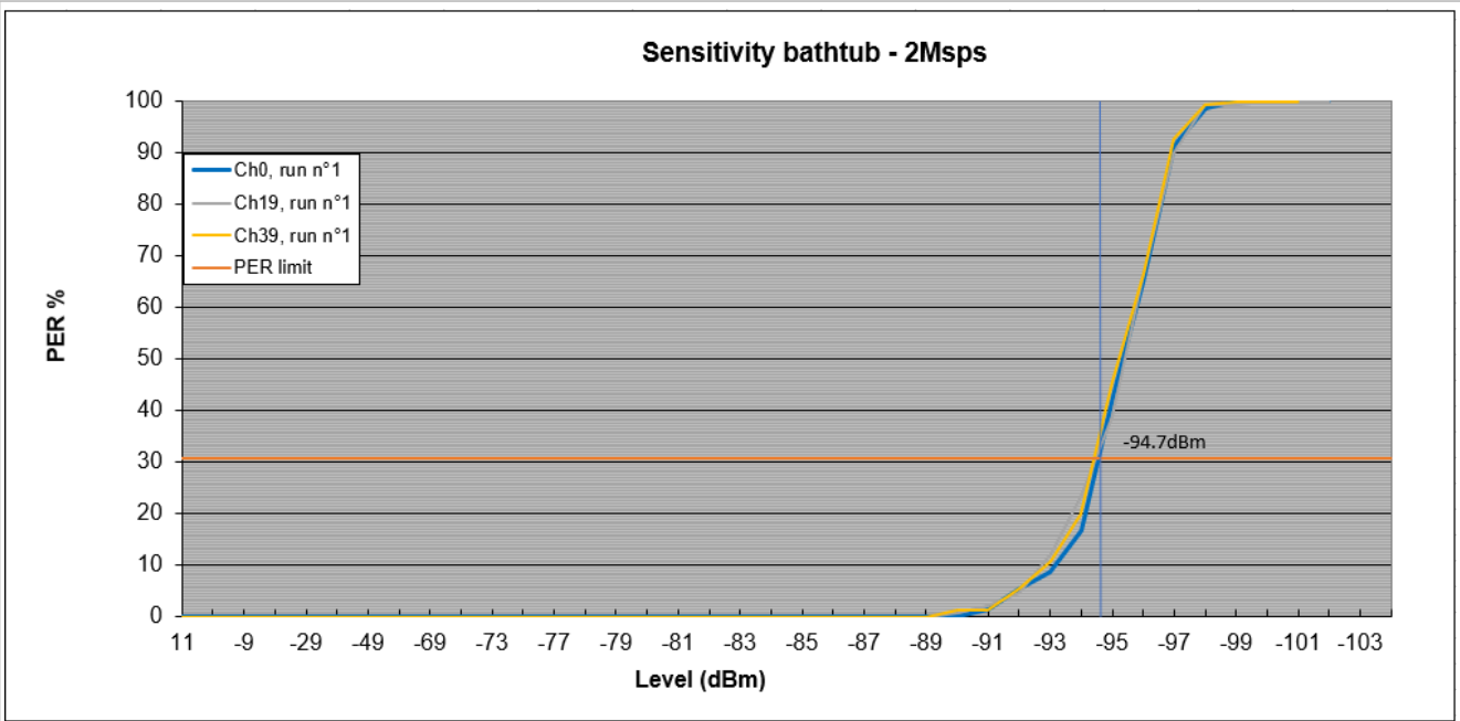
Figure 51. Sensitivity bathtub result – 2 Msps
