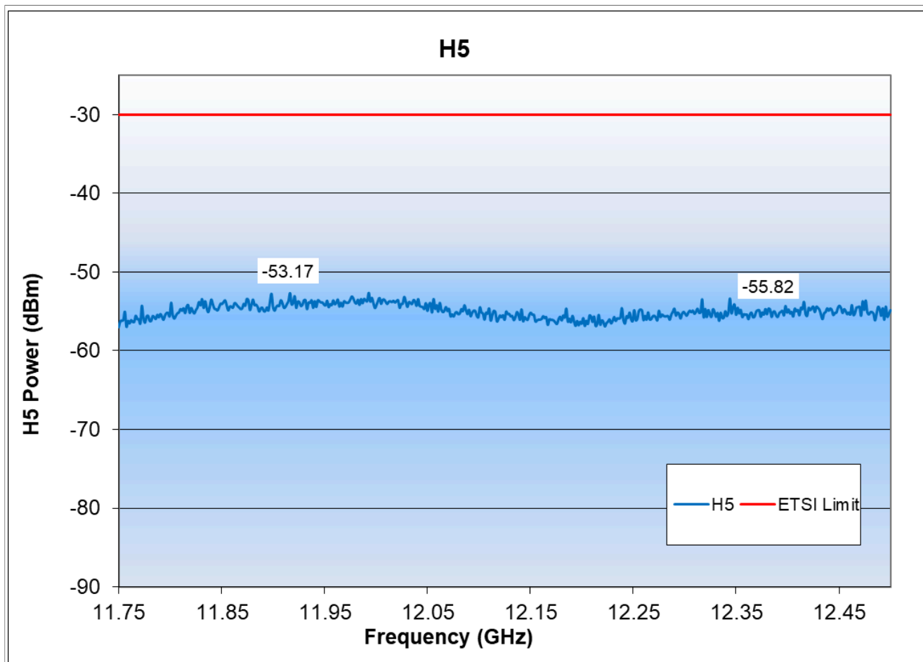
Figure 16. Bluetooth LE - Conducted H5 spurious
