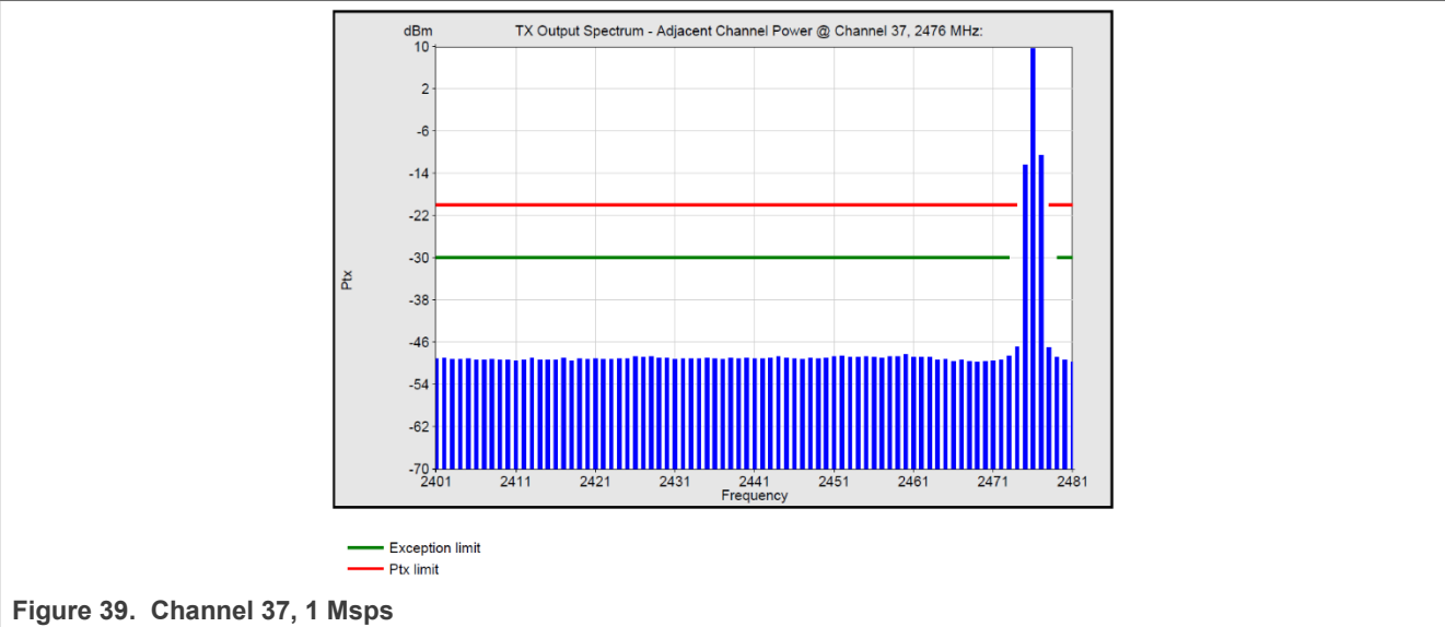
Figure 39. Channel 37, 1 Msps
