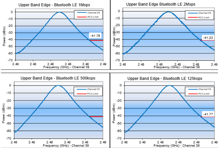
Figure 36. Out of band – Channel 39 - ARIB
