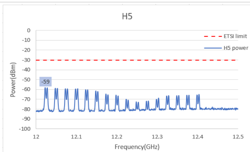
Figure 94. Conducted H5 spurious
