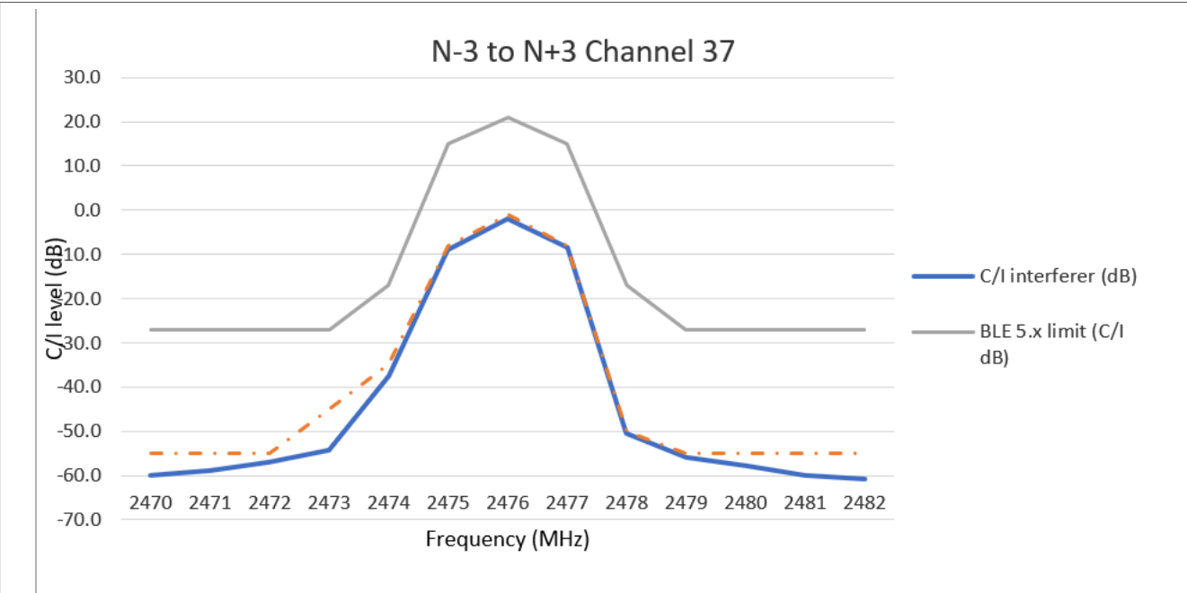
Figure 72. Adjacent, alternate, and co-channel rejection Bluetooth LE @125 ksps (LR S = 8) channel 37
