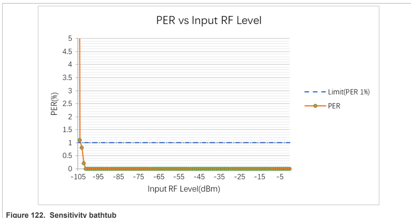
Figure 122. Sensitivity bathtub
