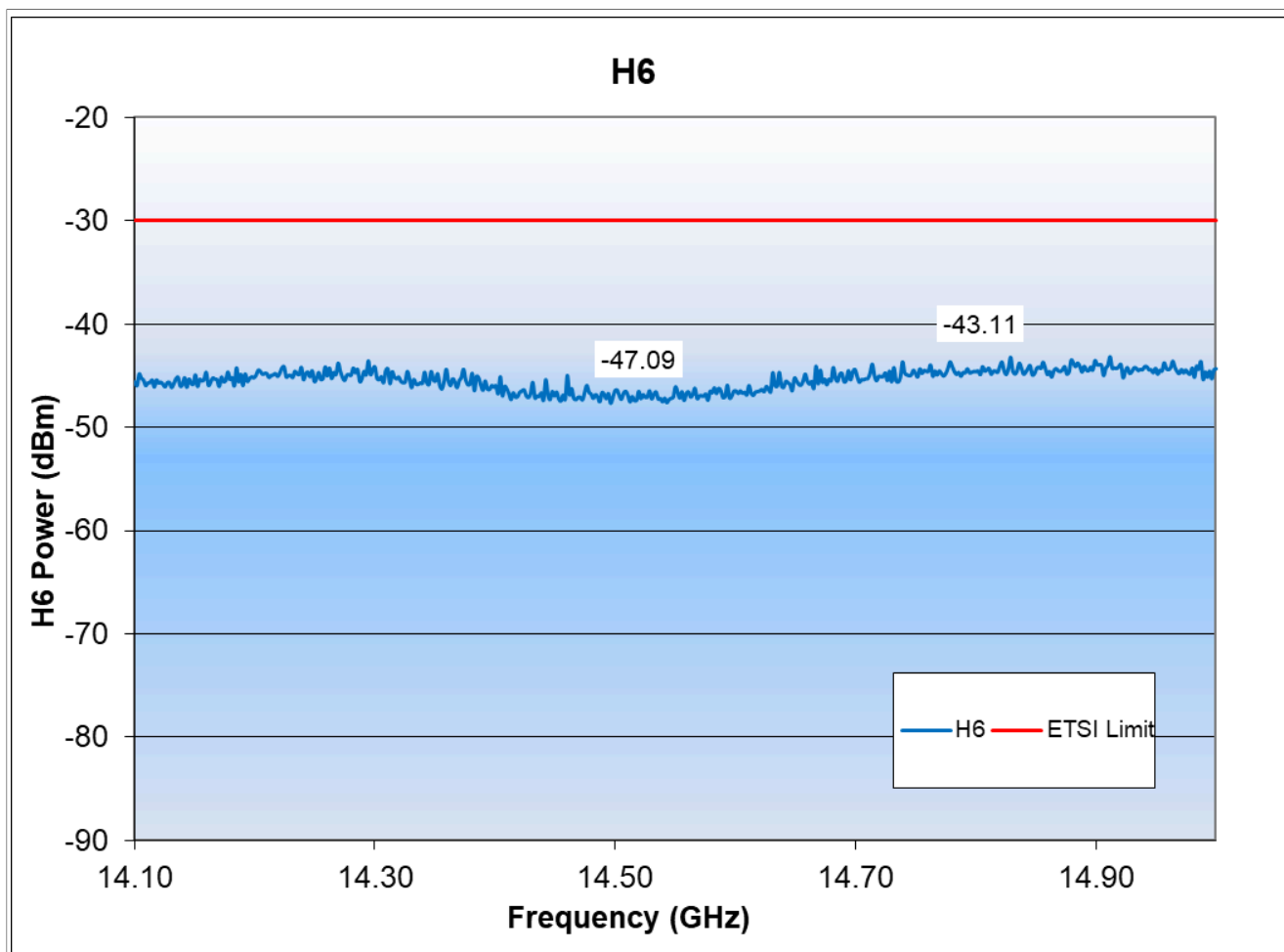
Figure 17. Bluetooth LE - Conducted H6 spurious
