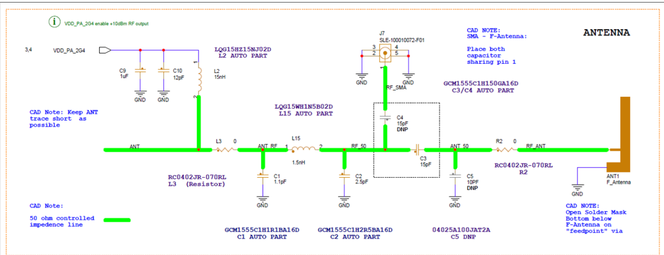
Figure 128. RF matching
