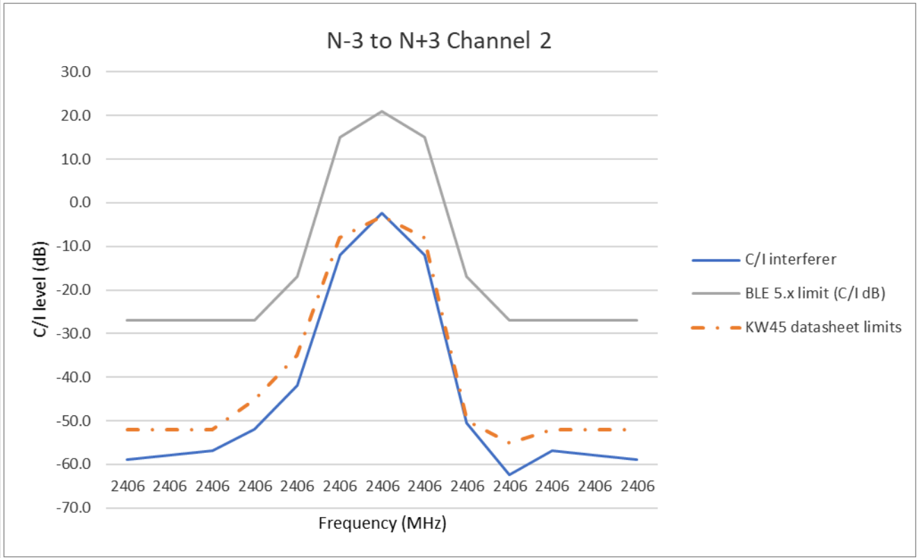
Figure 66. Adjacent, alternate, and co-channel rejection Bluetooth LE @500 kbps (LR S = 2) channel 2
