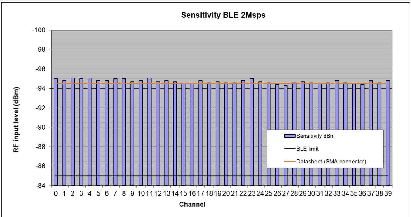
Figure 50. Sensitivity result – 2 Msps
