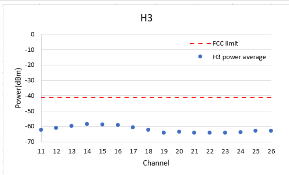
Figure 101. Conducted H3 spurious
