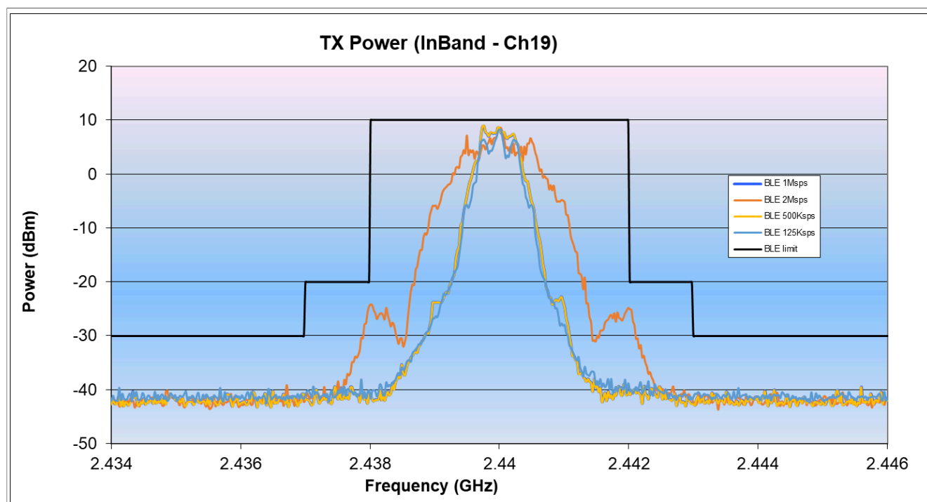
Figure 9. TX power in-band – Channel 19
