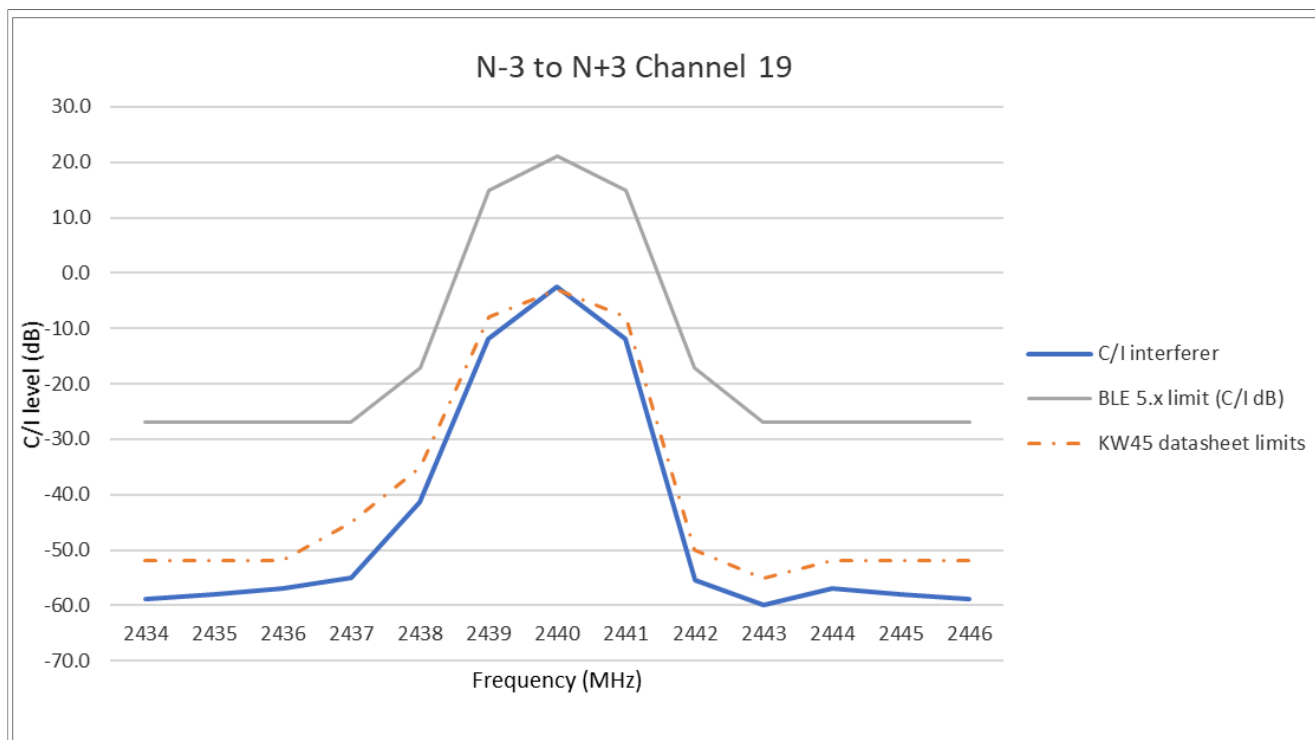
Figure 67. Adjacent, alternate, and co-channel rejection Bluetooth LE @500 kbps (LR S = 2) channel 19
