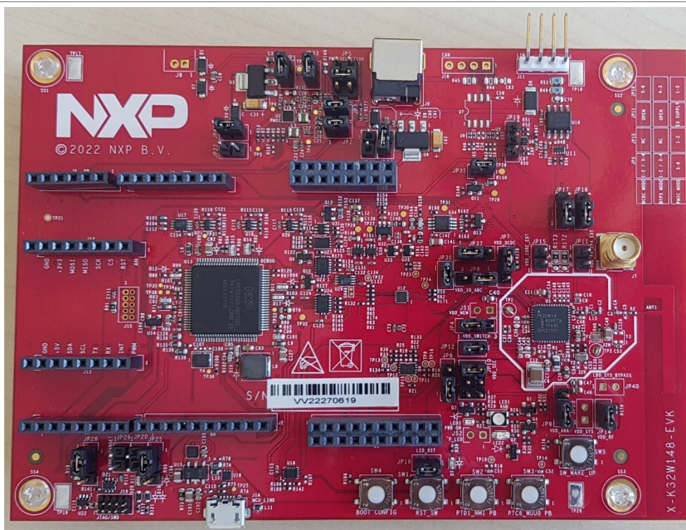
Figure 2. K32W148-EVK top-side view
