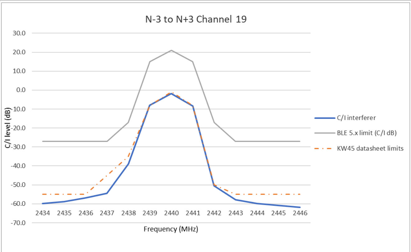
Figure 71. Adjacent, alternate, and co-channel rejection Bluetooth LE @125 ksps (LR S = 8) channel 19
