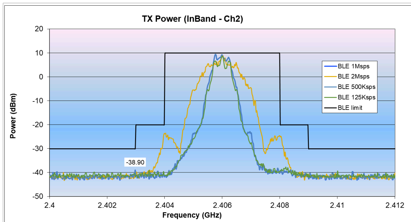
Figure 8. TX power in-band – Channel 2
