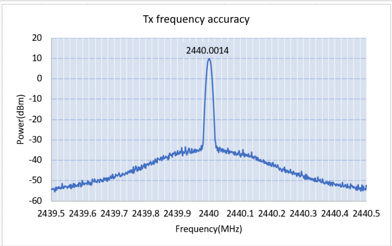
Figure 84. Frequency accuracy
