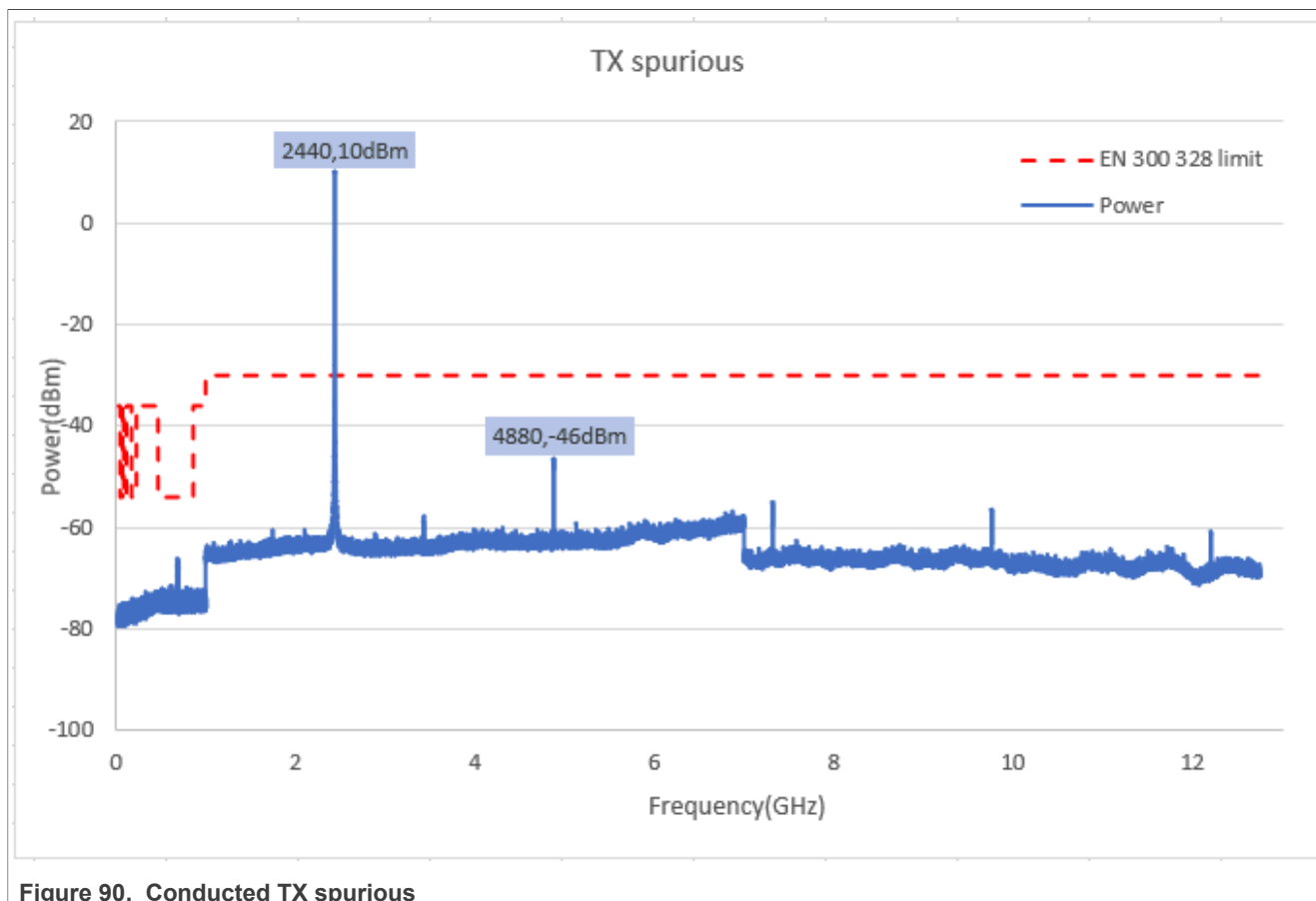
Figure 90. Conducted TX spurious
