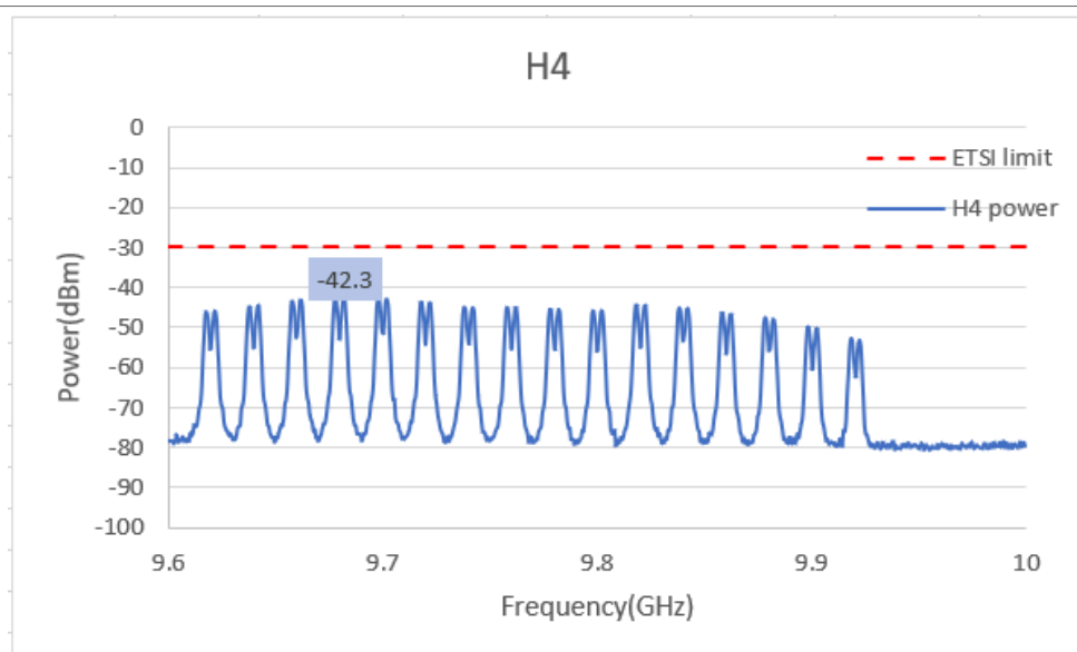
Figure 93. Conducted H4 spurious
