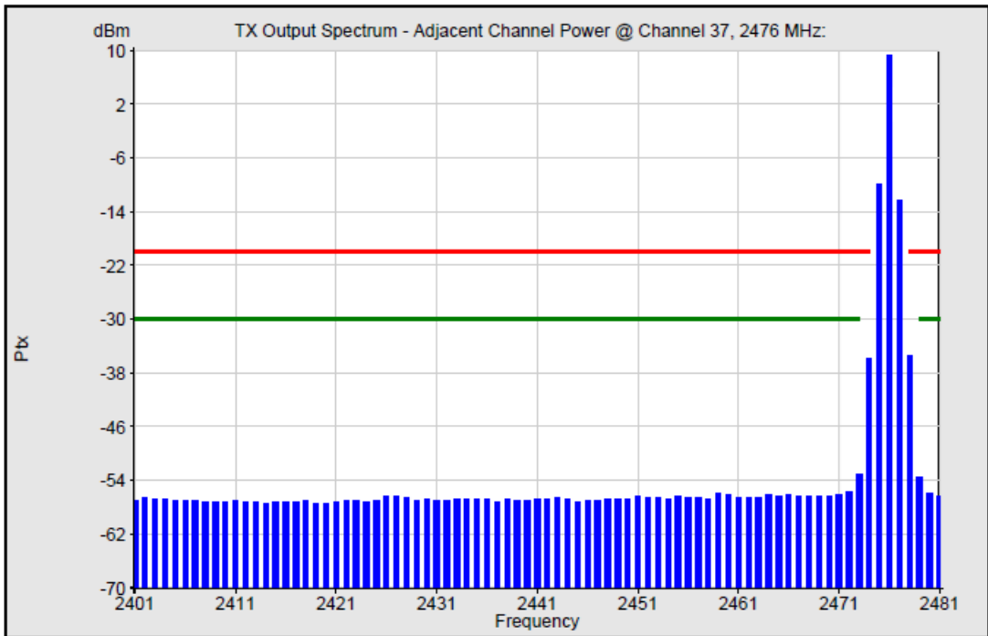
Figure 42. Channel 37, 2 Msps
