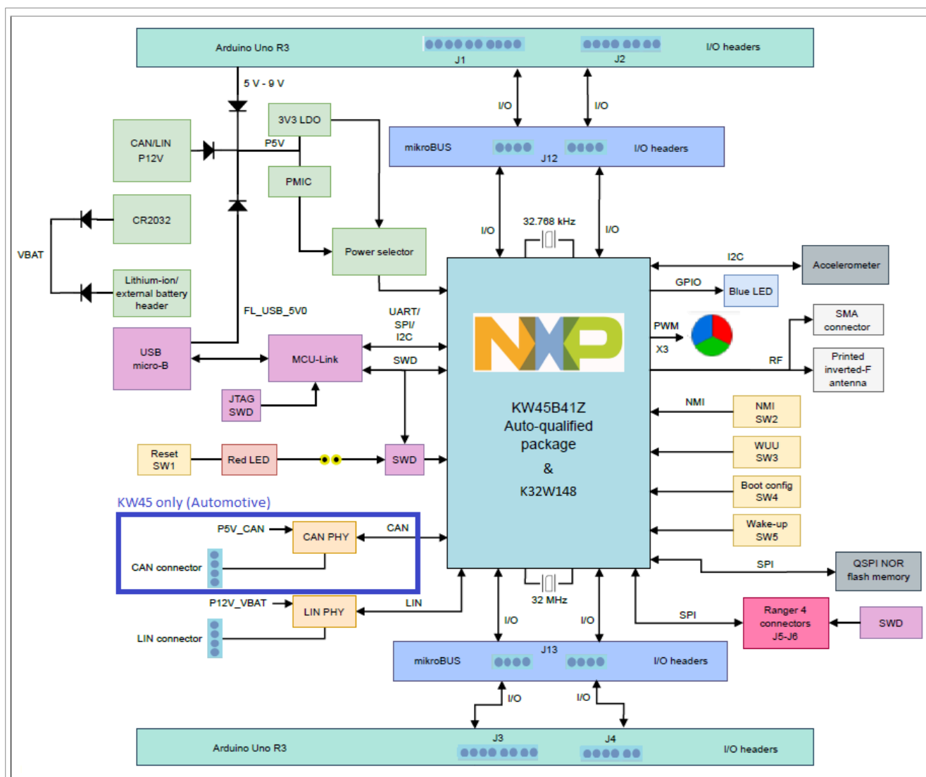
Figure 1. K32W148-EVK block diagram
