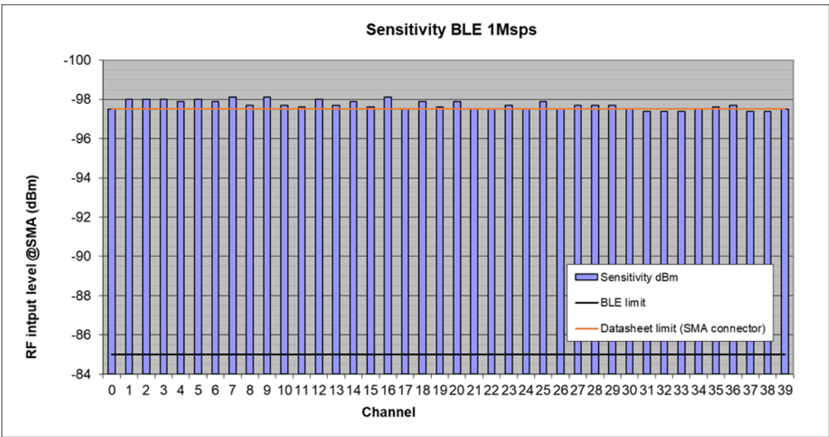
Figure 48. Sensitivity result – 1 Msps
