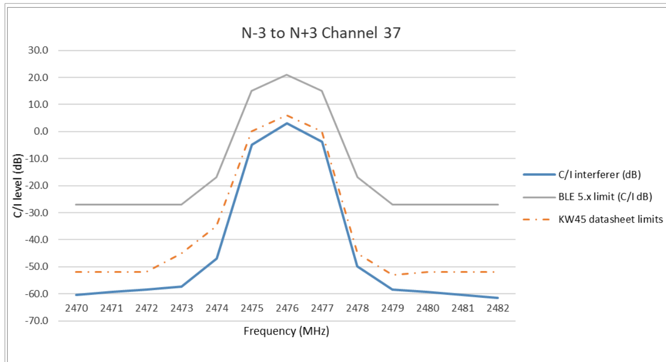
Figure 60. Adjacent, alternate, and co-channel rejection Bluetooth LE @1 Msps channel 37
