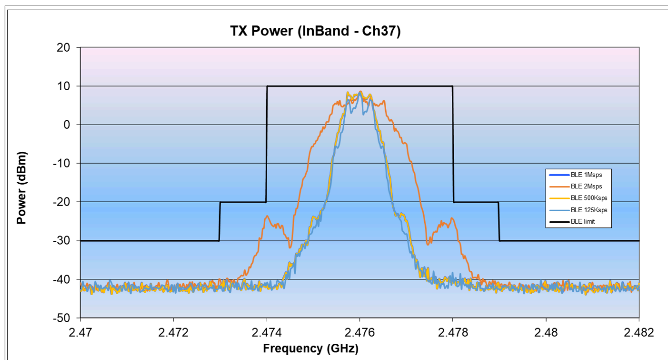
Figure 10. TX power in-band – Channel 37
