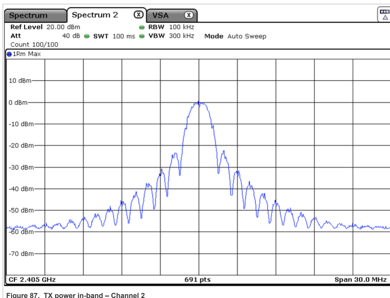
Figure 87. TX power in-band – Channel 2
