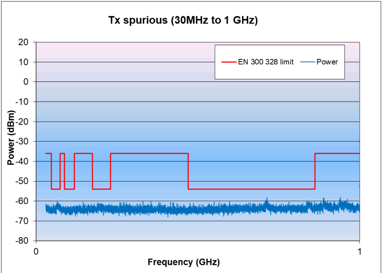
Figure 12. Bluetooth LE - Zoom In - Conducted TX spurious (30 MHz to 1 GHz)
