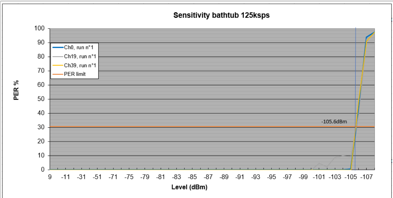
Figure 55. Sensitivity bathtub result – 125 ksps
