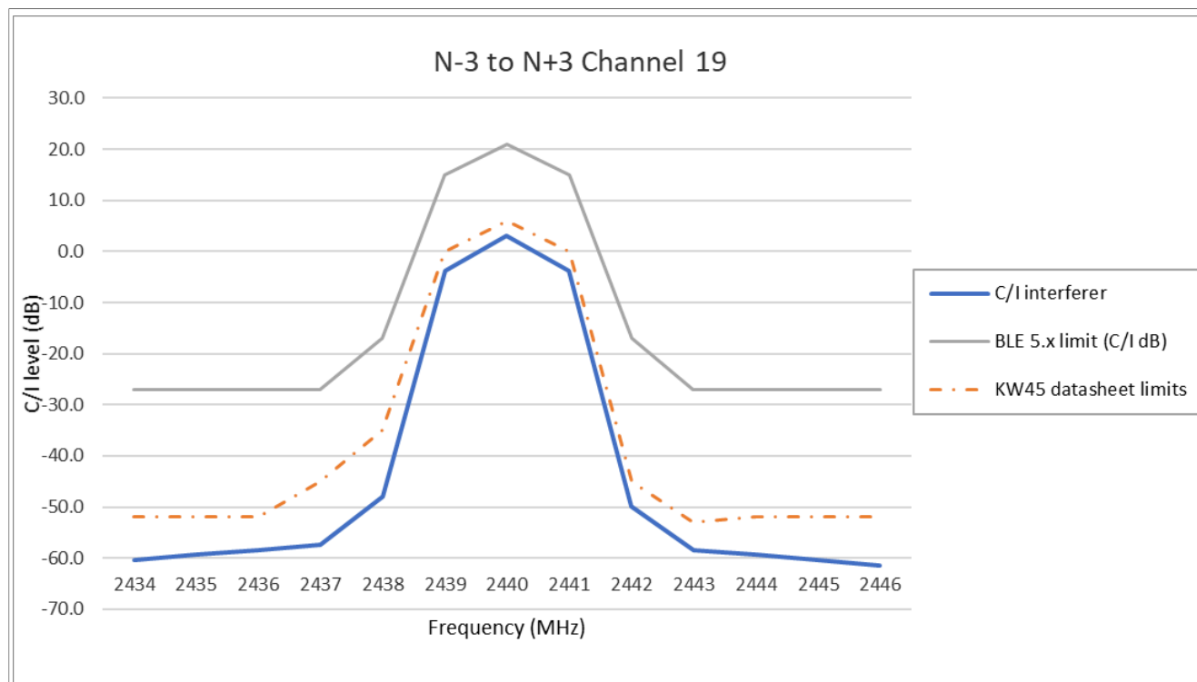
Figure 59. Adjacent, alternate, and co-channel rejection Bluetooth LE @1 Msps channel 19
