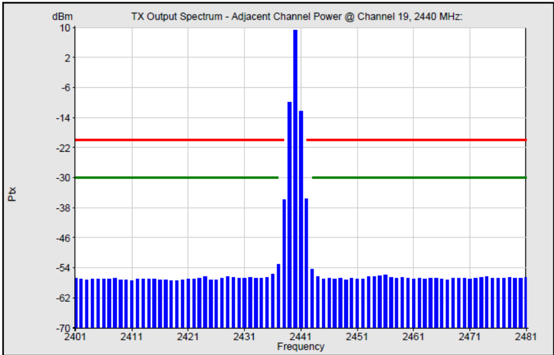
Figure 41. Channel 19, 2 Msps
