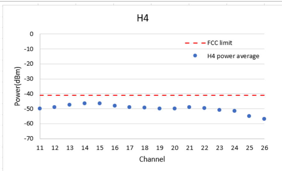
Figure 102. Conducted H4 spurious
