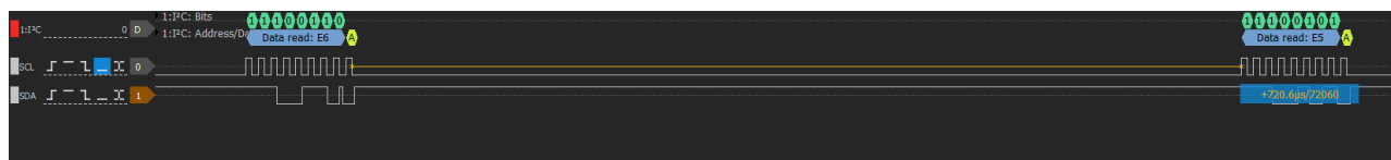
Figure 3. Enabling clock stretching before sending data
