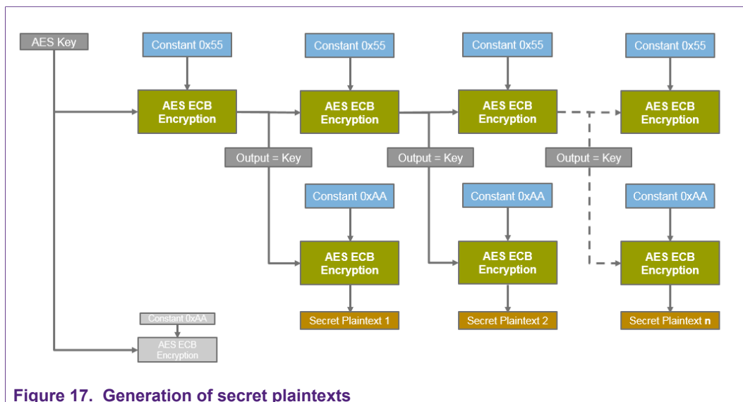
Figure 17. Generation of secret plaintexts
