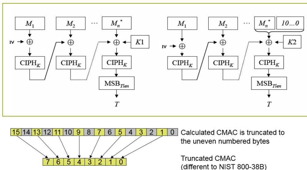
Figure 5. CMAC Calculation and Truncation for AES Secure Messaging
