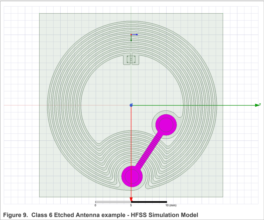
Figure 9. Class 6 Etched Antenna example - HFSS Simulation Model
