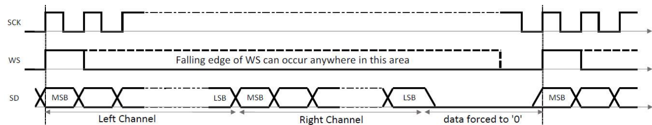
Figure 5. DSP format
