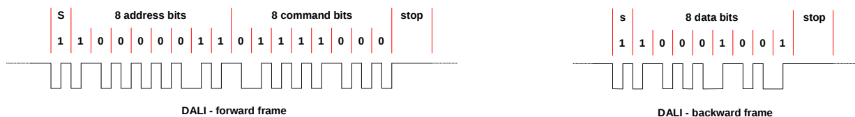
Fig 2. DALI forward and backward frame format
